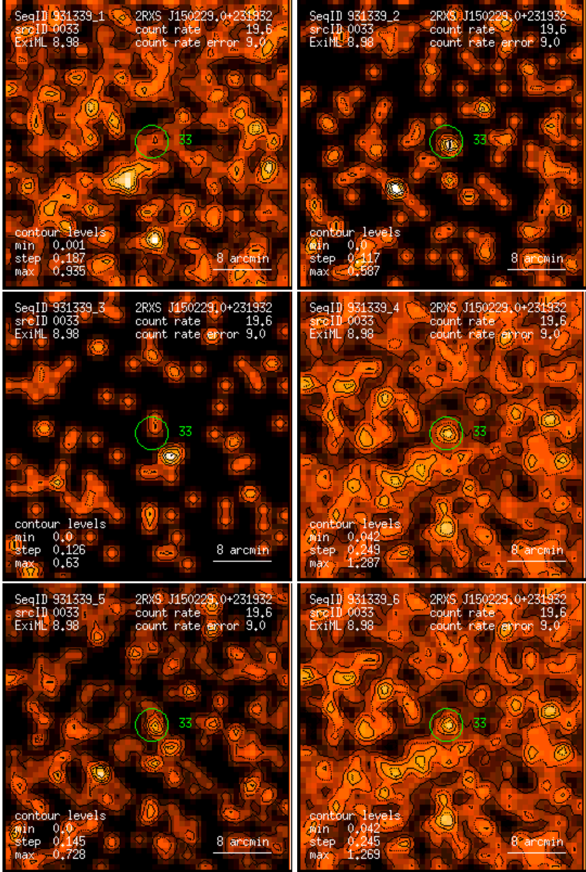
Figure 33: RASS 931339: detection 0033: band rate images, Gaussian filter: (1) PSPC channels 11 – 41, (2) 52 – 90, (3) 91 – 201, (4) 11 – 235, (5) 52 – 201, (6) 11 – 201. Broad band rates in counts/ks. Band rate contour levels in counts/ks/arcmin 2 .
