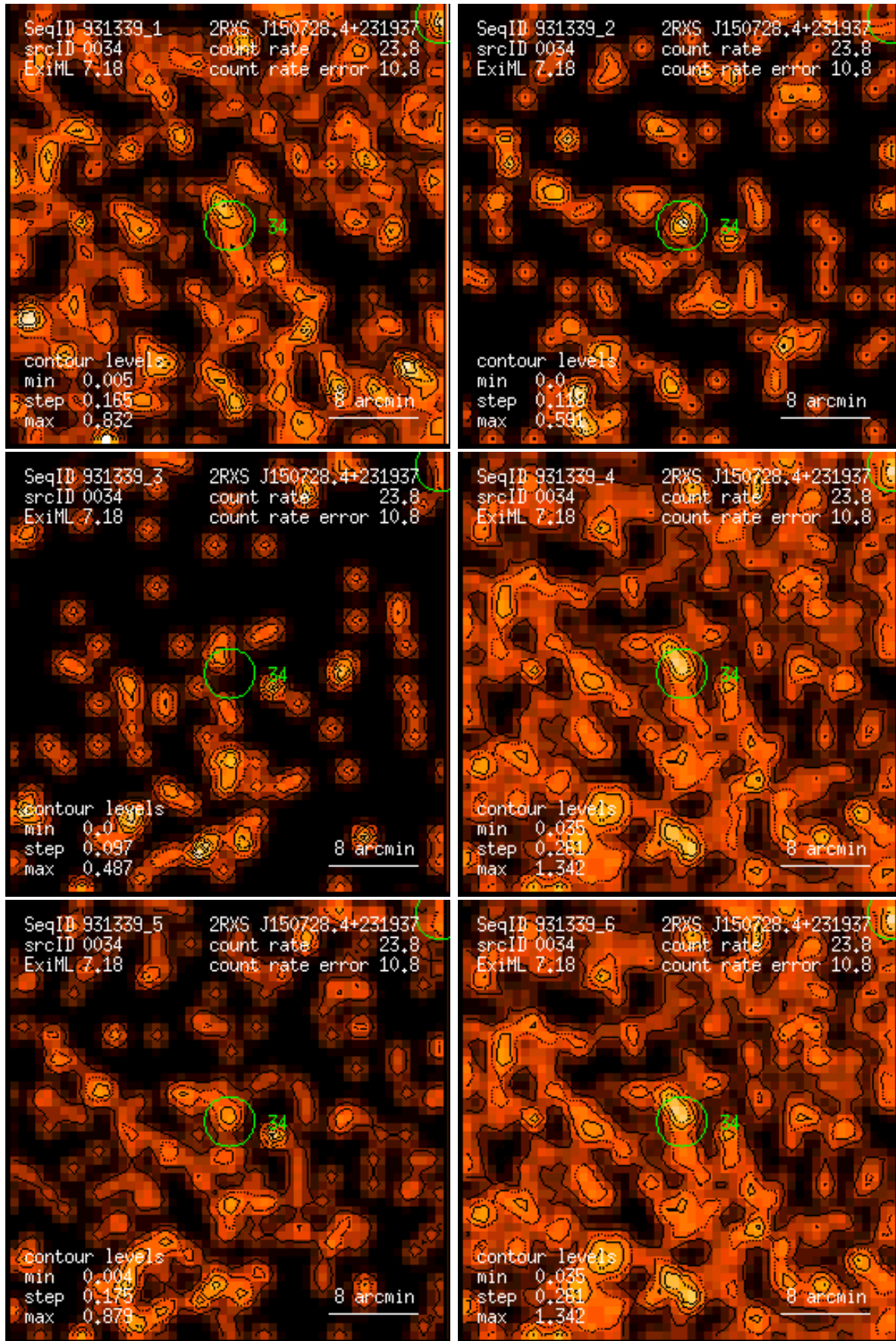
Figure 34: RASS 931339: detection 0034: band rate images, Gaussian filter: (1) PSPC channels 11 – 41, (2) 52 – 90, (3) 91 – 201, (4) 11 – 235, (5) 52 – 201, (6) 11 – 201. Broad band rates in counts/ks. Band rate contour levels in counts/ks/arcmin 2 .
