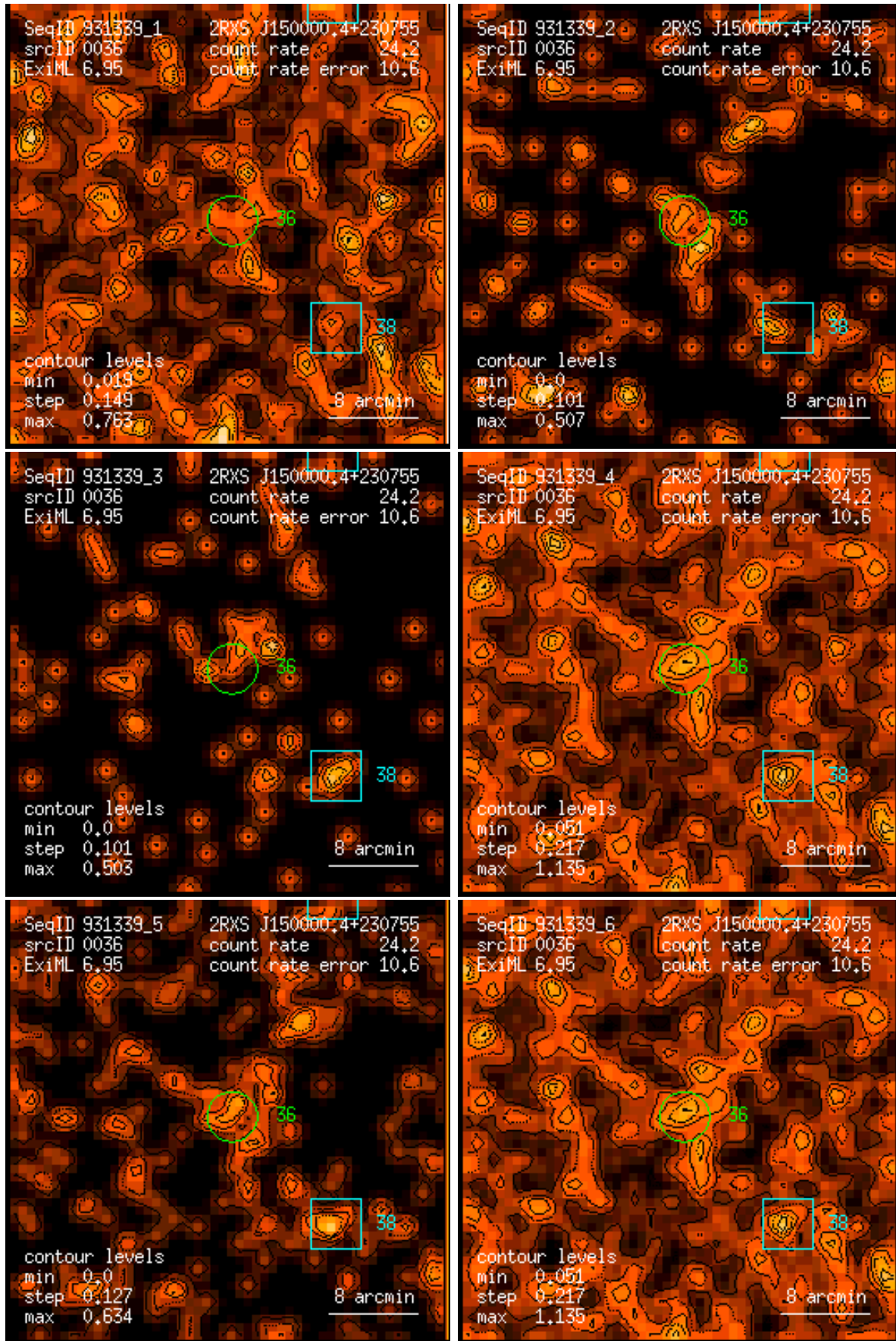
Figure 36: RASS 931339: detection 0036: band rate images, Gaussian filter: (1) PSPC channels 11 – 41, (2) 52 – 90, (3) 91 – 201, (4) 11 – 235, (5) 52 – 201, (6) 11 – 201. Broad band rates in counts/ks. Band rate contour levels in counts/ks/arcmin 2 .
