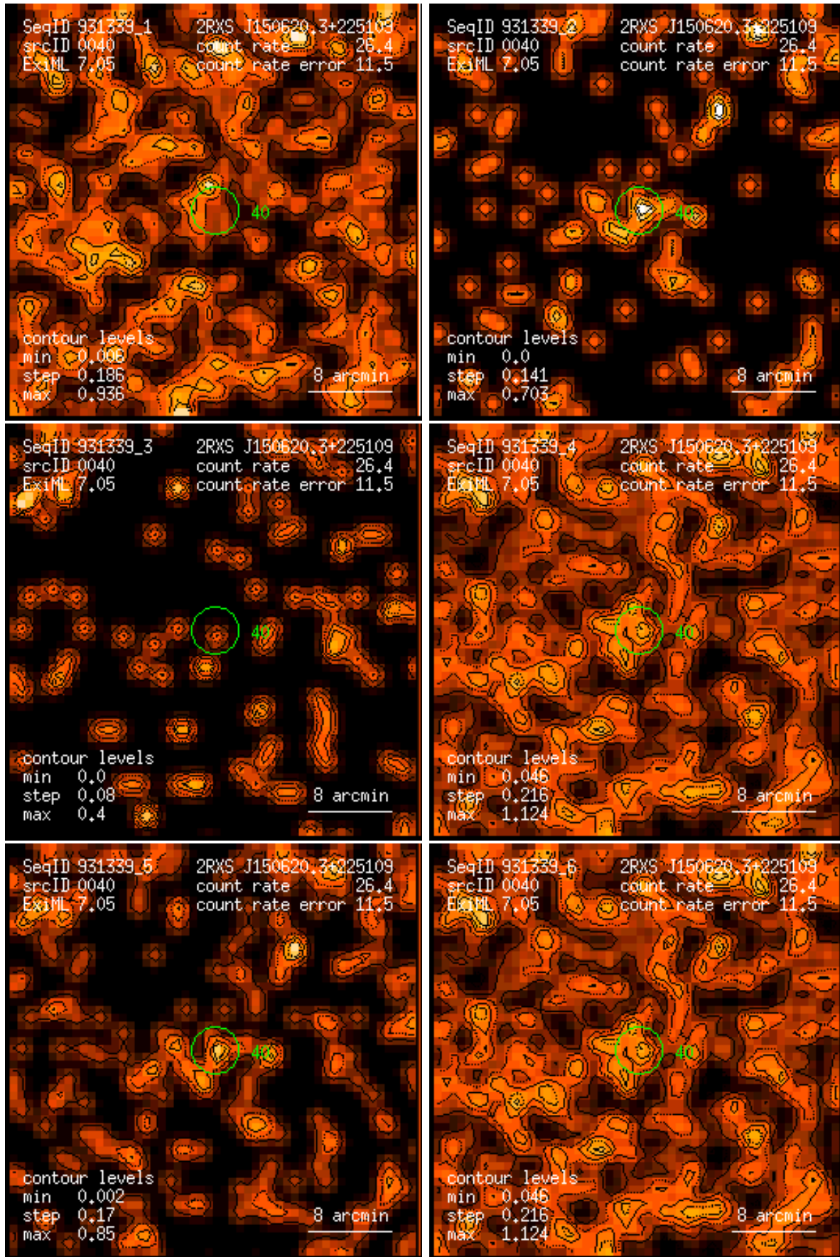
Figure 40: RASS 931339: detection 0040: band rate images, Gaussian filter: (1) PSPC channels 11 – 41, (2) 52 – 90, (3) 91 – 201, (4) 11 – 235, (5) 52 – 201, (6) 11 – 201. Broad band rates in counts/ks. Band rate contour levels in counts/ks/arcmin 2 .
