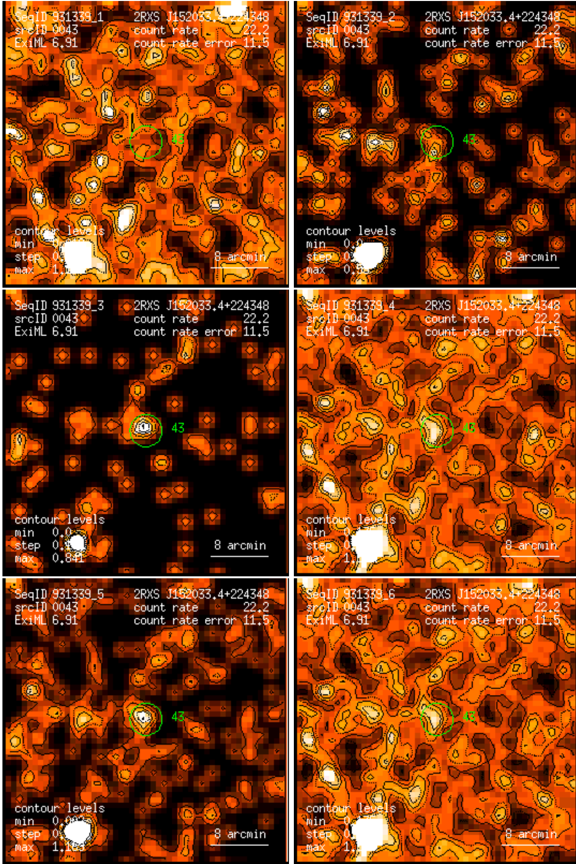
Figure 43: RASS 931339: detection 0043: band rate images, Gaussian filter: (1) PSPC channels 11 – 41, (2) 52 – 90, (3) 91 – 201, (4) 11 – 235, (5) 52 – 201, (6) 11 – 201. Broad band rates in counts/ks. Band rate contour levels in counts/ks/arcmin 2 .
