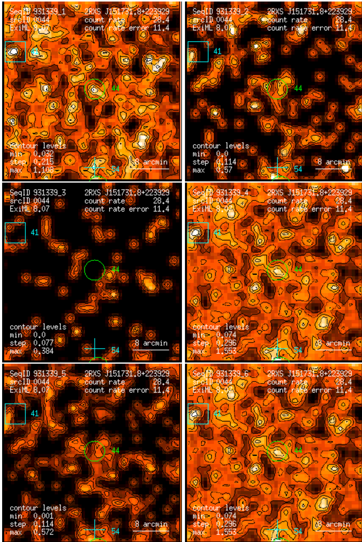
Figure 44: RASS 931339: detection 0044: band rate images, Gaussian filter: (1) PSPC channels 11 – 41, (2) 52 – 90, (3) 91 – 201, (4) 11 – 235, (5) 52 – 201, (6) 11 – 201. Broad band rates in counts/ks. Band rate contour levels in counts/ks/arcmin 2 .
