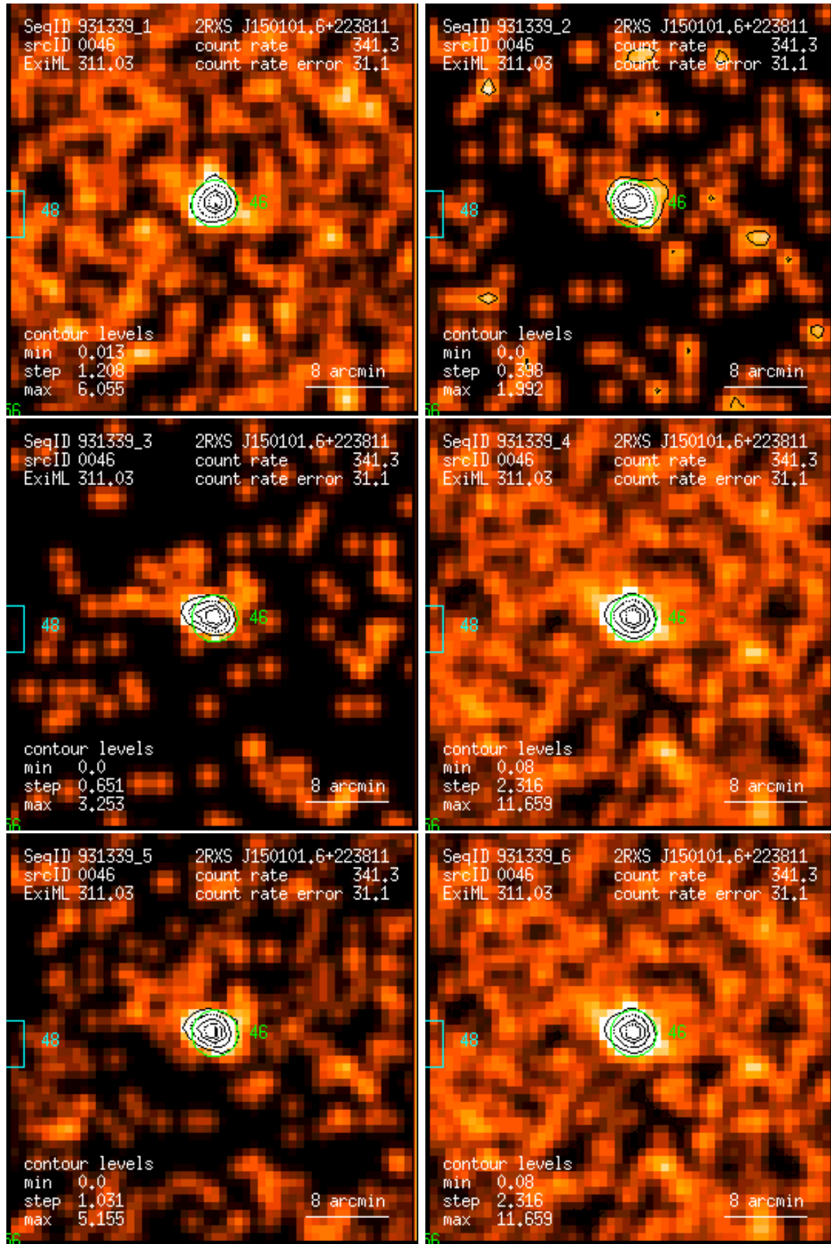
Figure 46: RASS 931339: detection 0046: band rate images, Gaussian filter: (1) PSPC channels 11 – 41, (2) 52 – 90, (3) 91 – 201, (4) 11 – 235, (5) 52 – 201, (6) 11 – 201. Broad band rates in counts/ks. Band rate contour levels in counts/ks/arcmin 2 .
