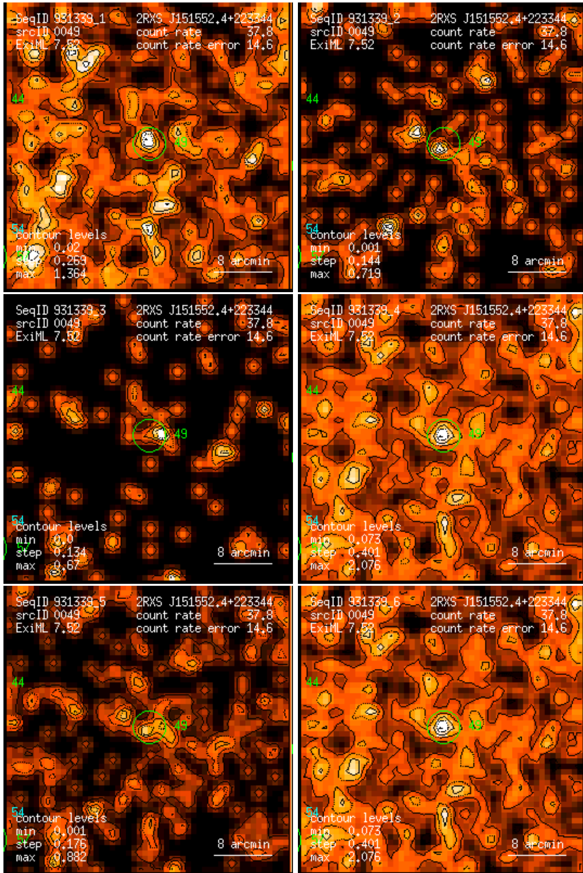
Figure 49: RASS 931339: detection 0049: band rate images, Gaussian filter: (1) PSPC channels 11 – 41, (2) 52 – 90, (3) 91 – 201, (4) 11 – 235, (5) 52 – 201, (6) 11 – 201. Broad band rates in counts/ks. Band rate contour levels in counts/ks/arcmin 2 .
