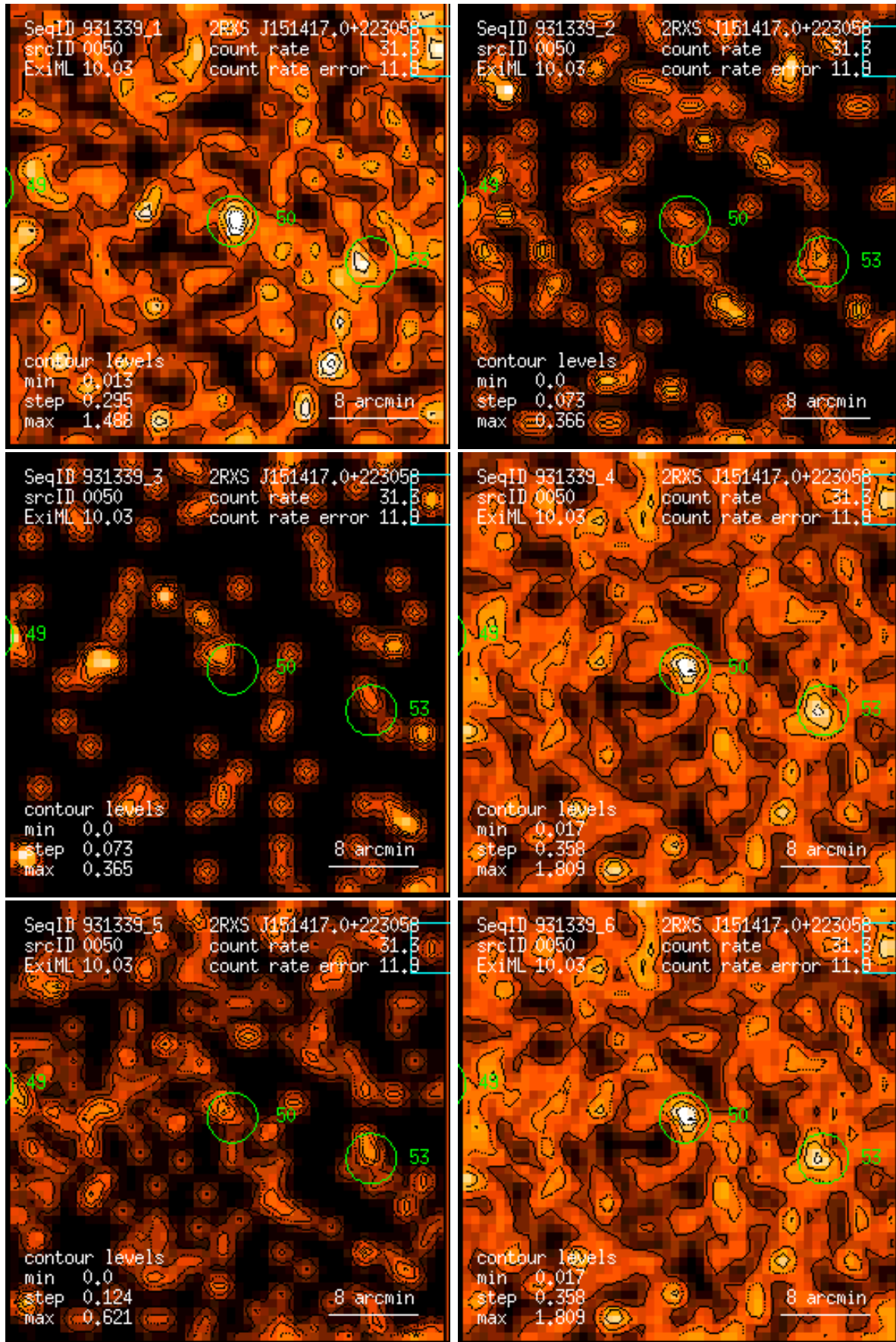
Figure 50: RASS 931339: detection 0050: band rate images, Gaussian filter: (1) PSPC channels 11 – 41, (2) 52 – 90, (3) 91 – 201, (4) 11 – 235, (5) 52 – 201, (6) 11 – 201. Broad band rates in counts/ks. Band rate contour levels in counts/ks/arcmin 2 .
