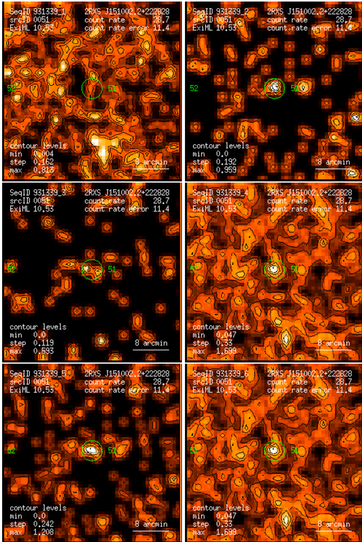
Figure 51: RASS 931339: detection 0051: band rate images, Gaussian filter: (1) PSPC channels 11 – 41, (2) 52 – 90, (3) 91 – 201, (4) 11 – 235, (5) 52 – 201, (6) 11 – 201. Broad band rates in counts/ks. Band rate contour levels in counts/ks/arcmin 2 .
