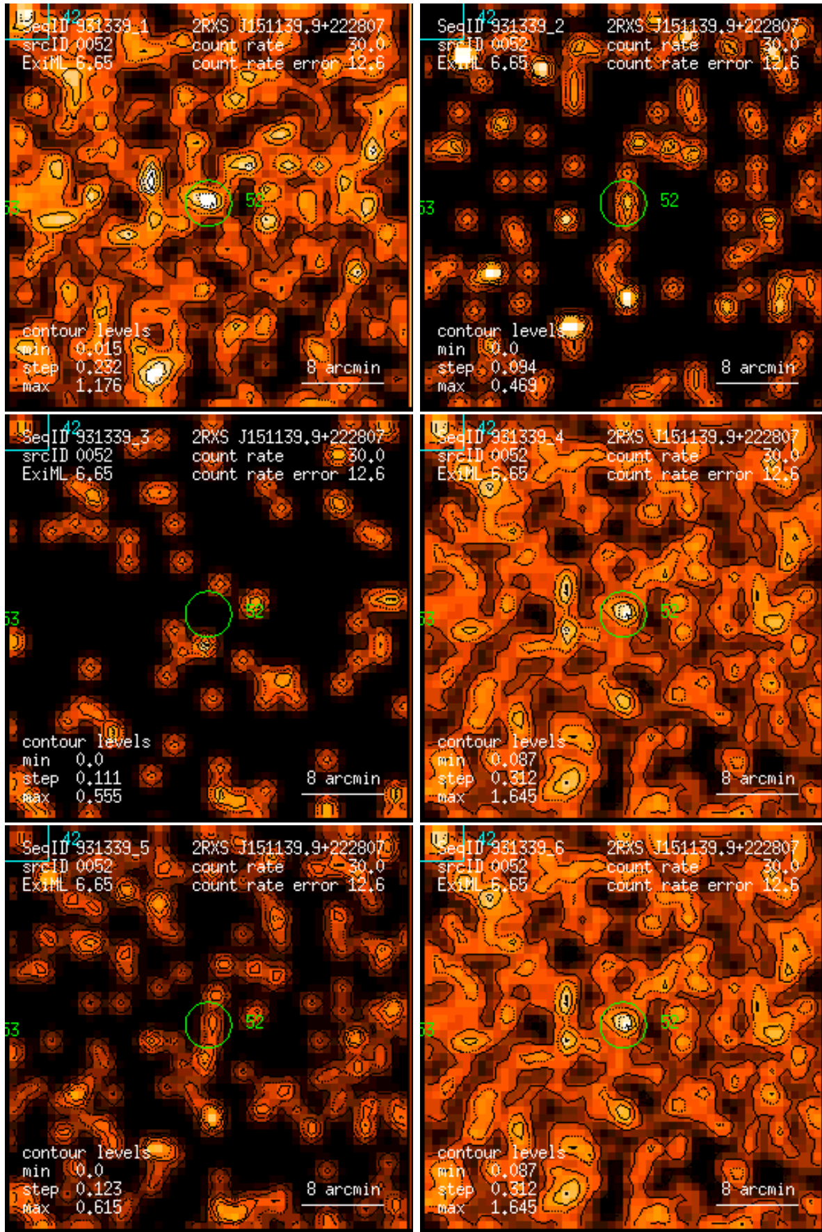
Figure 52: RASS 931339: detection 0052: band rate images, Gaussian filter: (1) PSPC channels 11 – 41, (2) 52 – 90, (3) 91 – 201, (4) 11 – 235, (5) 52 – 201, (6) 11 – 201. Broad band rates in counts/ks. Band rate contour levels in counts/ks/arcmin 2 .
