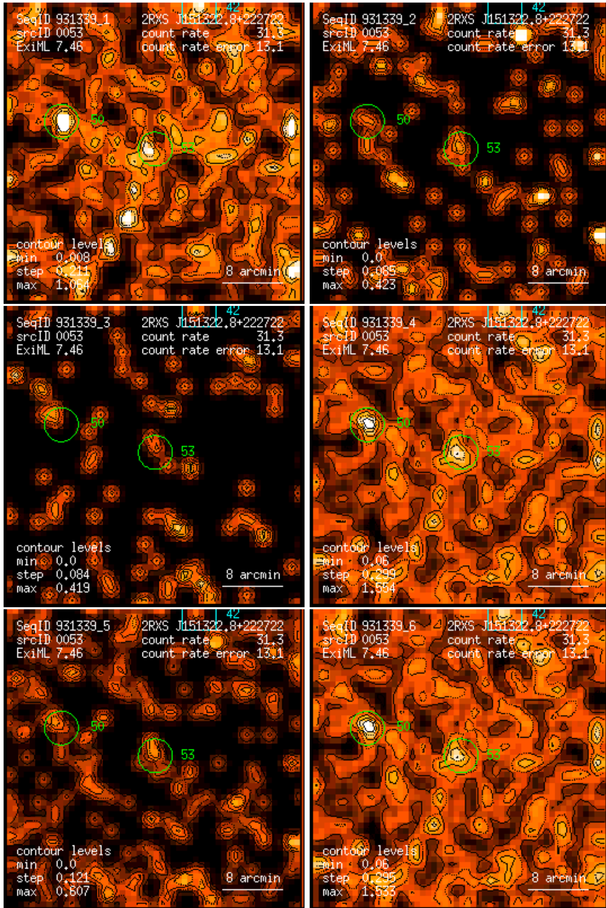
Figure 53: RASS 931339: detection 0053: band rate images, Gaussian filter: (1) PSPC channels 11 – 41, (2) 52 – 90, (3) 91 – 201, (4) 11 – 235, (5) 52 – 201, (6) 11 – 201. Broad band rates in counts/ks. Band rate contour levels in counts/ks/arcmin 2 .
