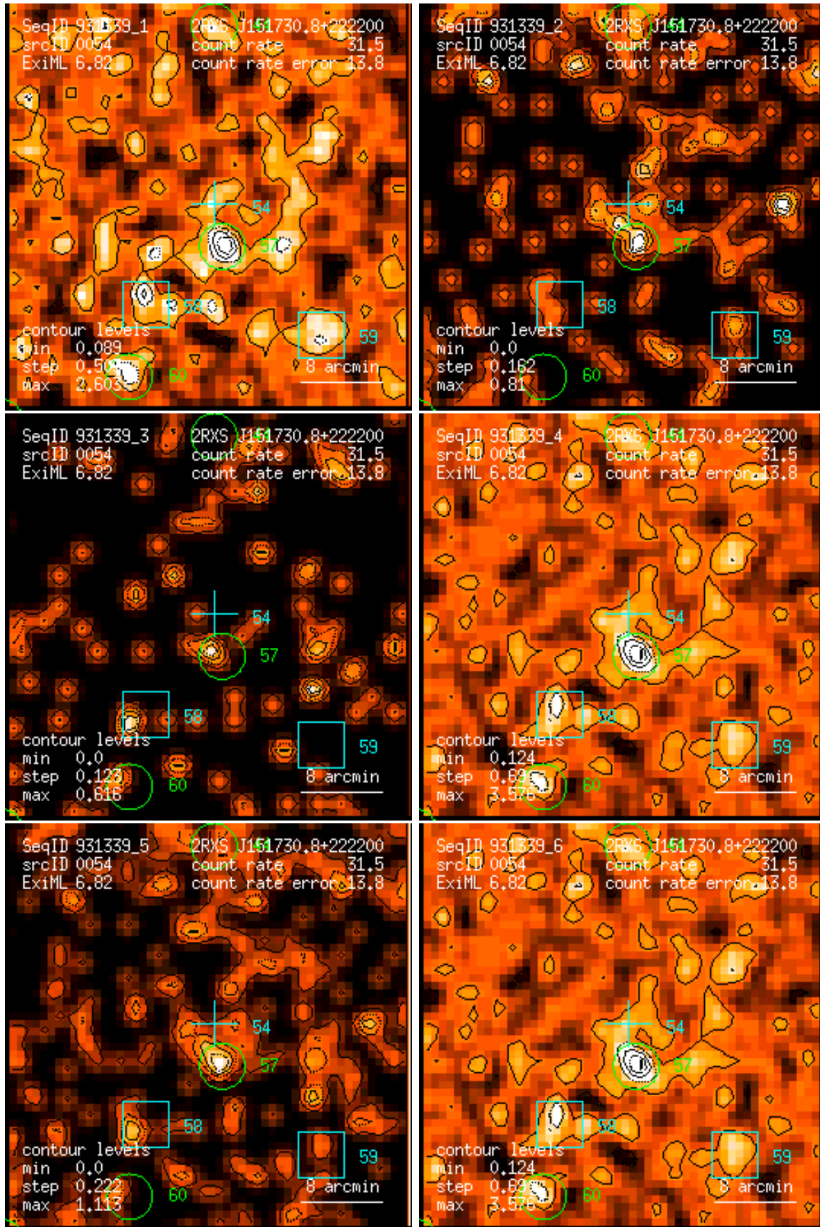
Figure 54: RASS 931339: detection 0054: band rate images, Gaussian filter: (1) PSPC channels 11 – 41, (2) 52 – 90, (3) 91 – 201, (4) 11 – 235, (5) 52 – 201, (6) 11 – 201. Broad band rates in counts/ks. Band rate contour levels in counts/ks/arcmin 2 .
