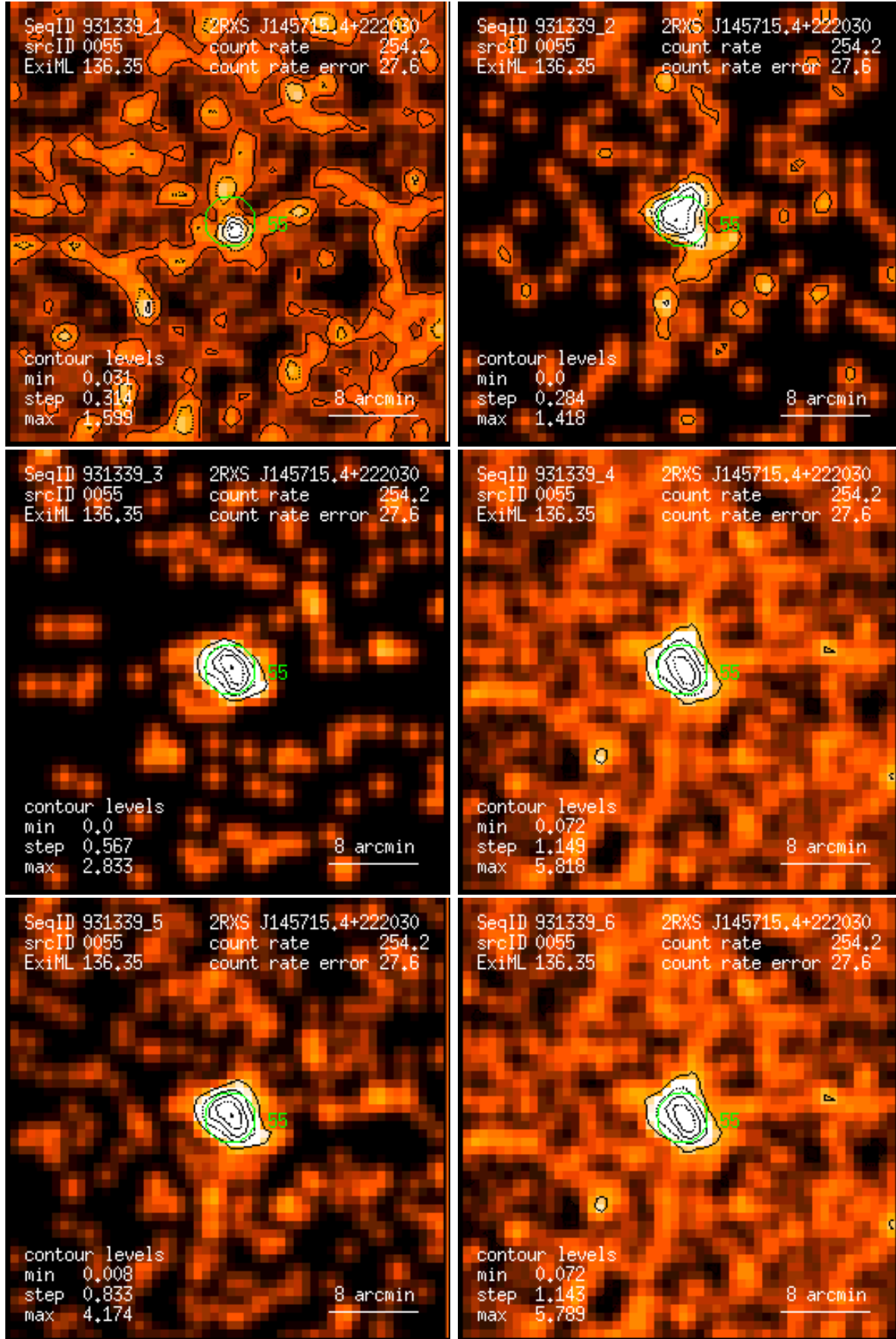
Figure 55: RASS 931339: detection 0055: band rate images, Gaussian filter: (1) PSPC channels 11 – 41, (2) 52 – 90, (3) 91 – 201, (4) 11 – 235, (5) 52 – 201, (6) 11 – 201. Broad band rates in counts/ks. Band rate contour levels in counts/ks/arcmin 2 .
