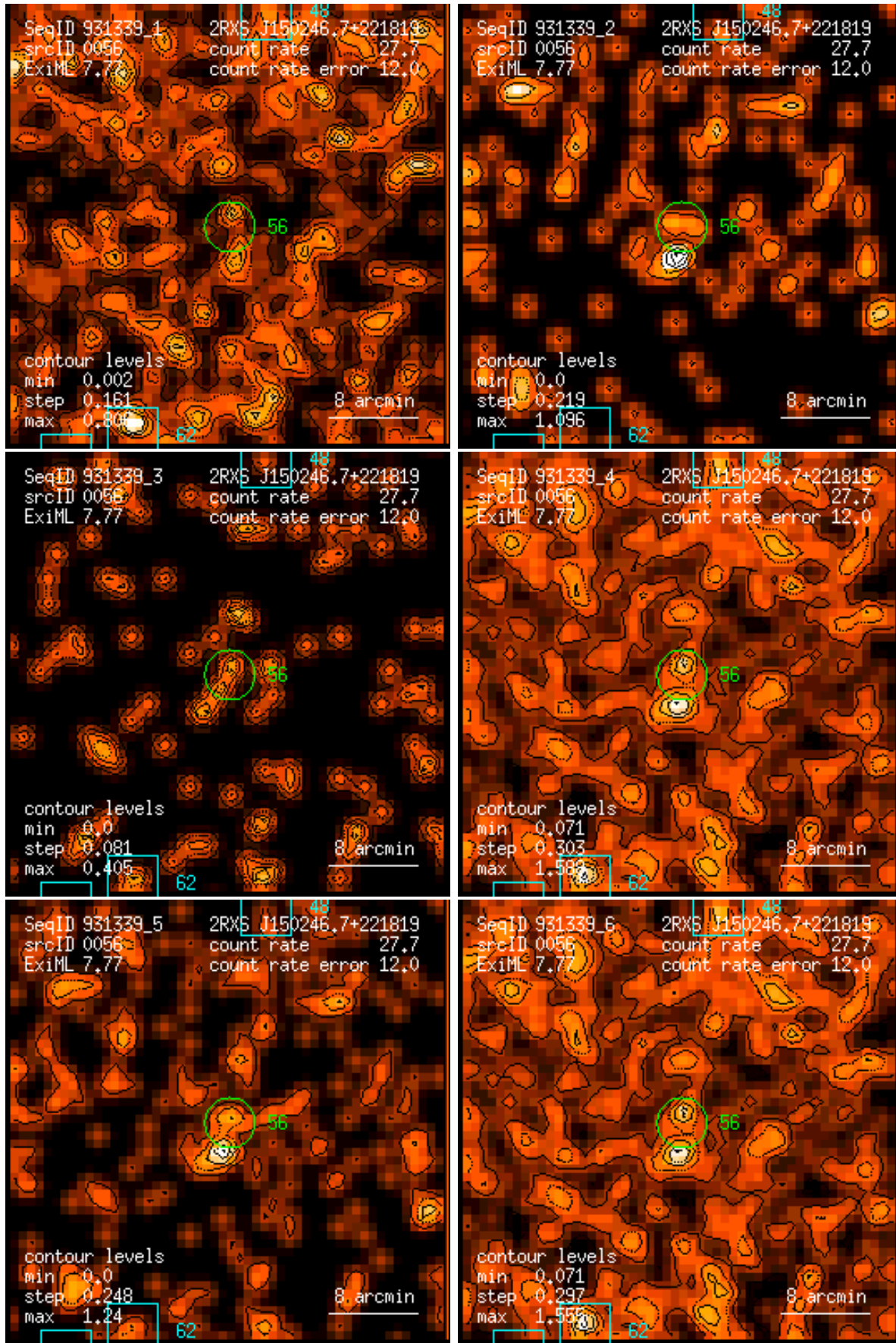
Figure 56: RASS 931339: detection 0056: band rate images, Gaussian filter: (1) PSPC channels 11 – 41, (2) 52 – 90, (3) 91 – 201, (4) 11 – 235, (5) 52 – 201, (6) 11 – 201. Broad band rates in counts/ks. Band rate contour levels in counts/ks/arcmin 2 .
