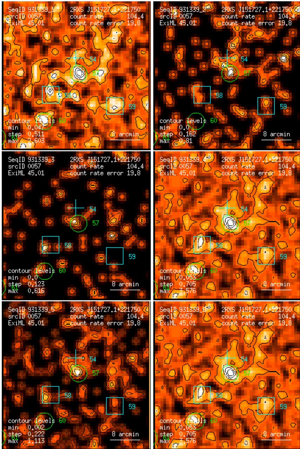
Figure 57: RASS 931339: detection 0057: band rate images, Gaussian filter: (1) PSPC channels 11 – 41, (2) 52 – 90, (3) 91 – 201, (4) 11 – 235, (5) 52 – 201, (6) 11 – 201. Broad band rates in counts/ks. Band rate contour levels in counts/ks/arcmin 2 .
