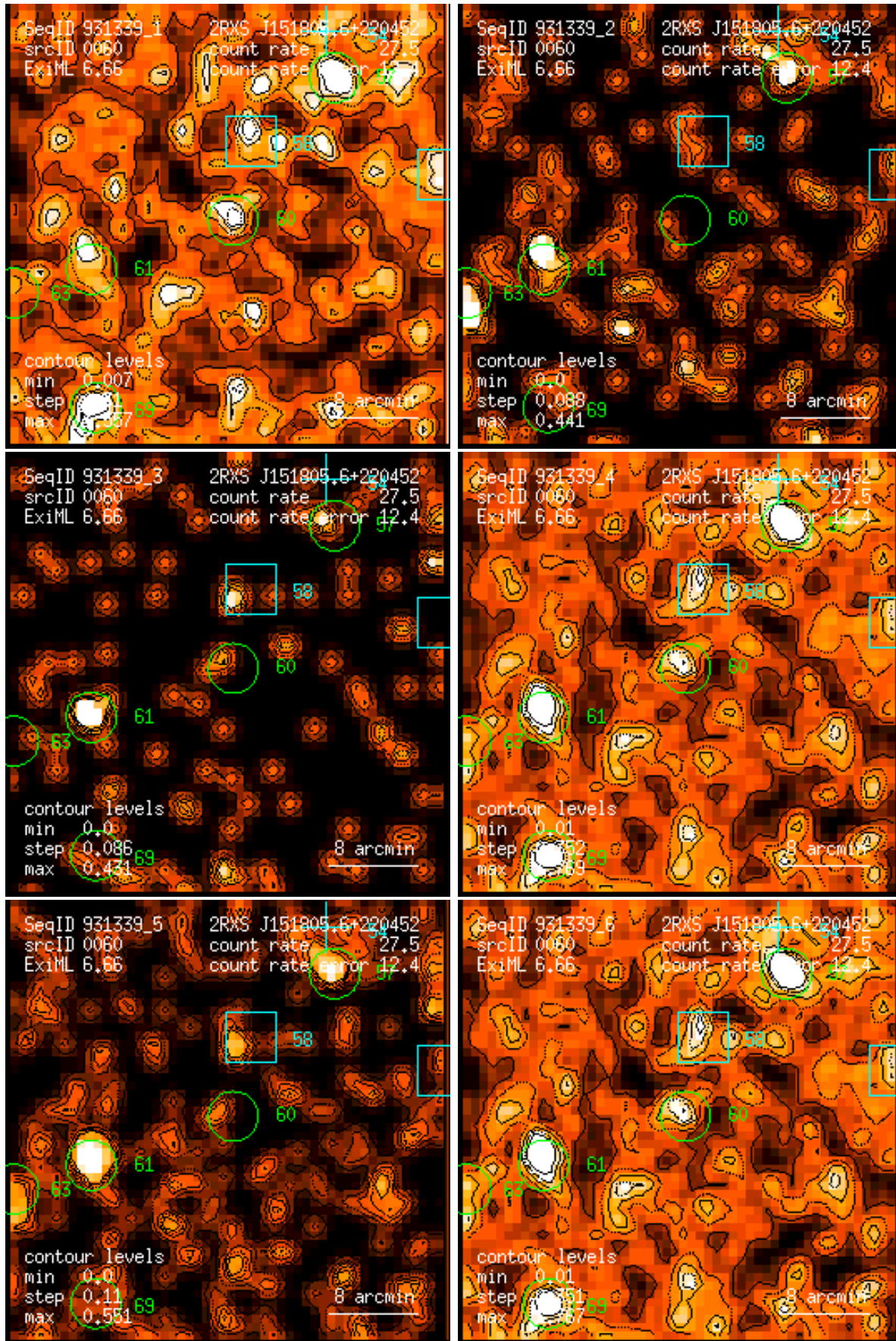
Figure 60: RASS 931339: detection 0060: band rate images, Gaussian filter: (1) PSPC channels 11 – 41, (2) 52 – 90, (3) 91 – 201, (4) 11 – 235, (5) 52 – 201, (6) 11 – 201. Broad band rates in counts/ks. Band rate contour levels in counts/ks/arcmin 2 .
