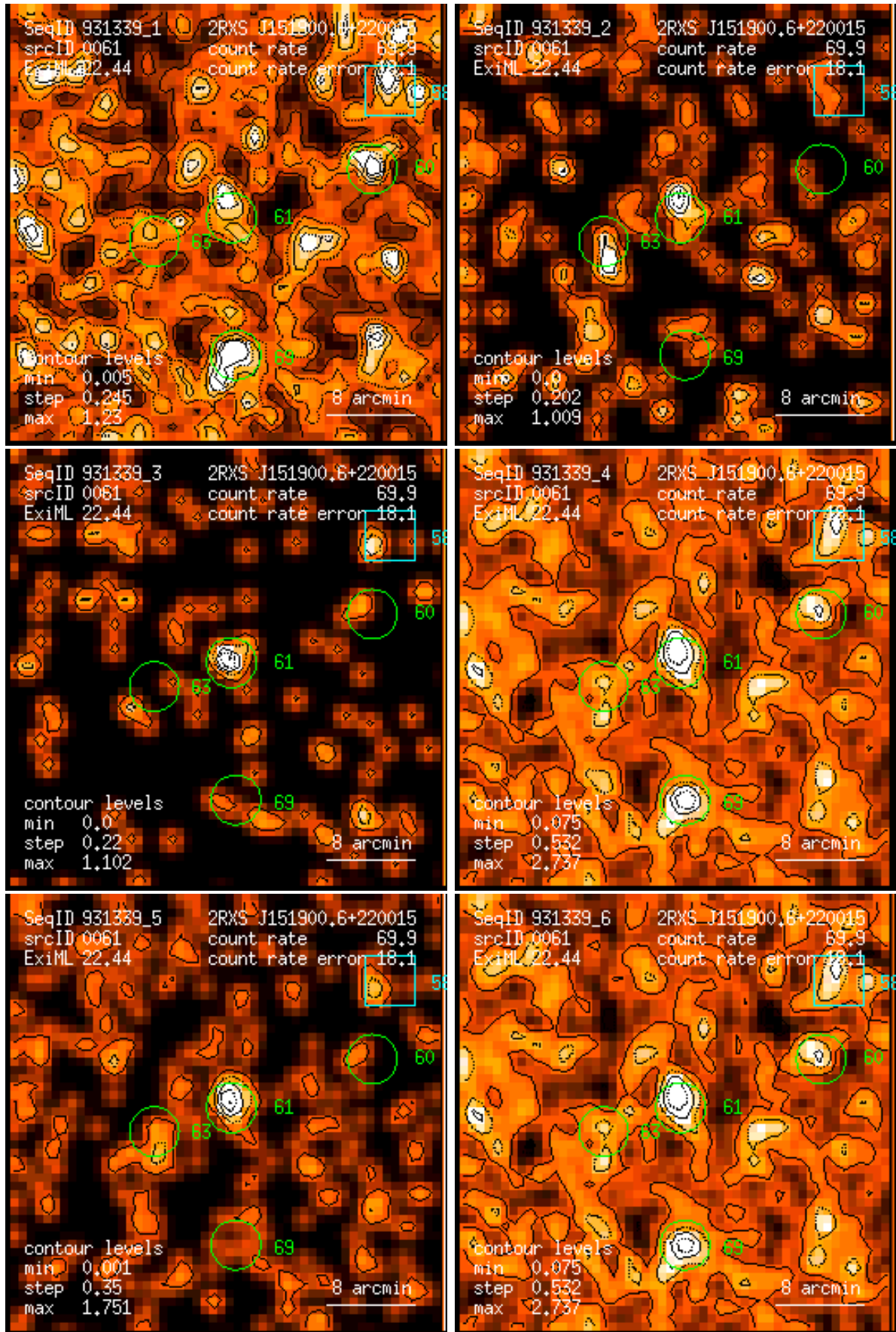
Figure 61: RASS 931339: detection 0061: band rate images, Gaussian filter: (1) PSPC channels 11 – 41, (2) 52 – 90, (3) 91 – 201, (4) 11 – 235, (5) 52 – 201, (6) 11 – 201. Broad band rates in counts/ks. Band rate contour levels in counts/ks/arcmin 2 .
