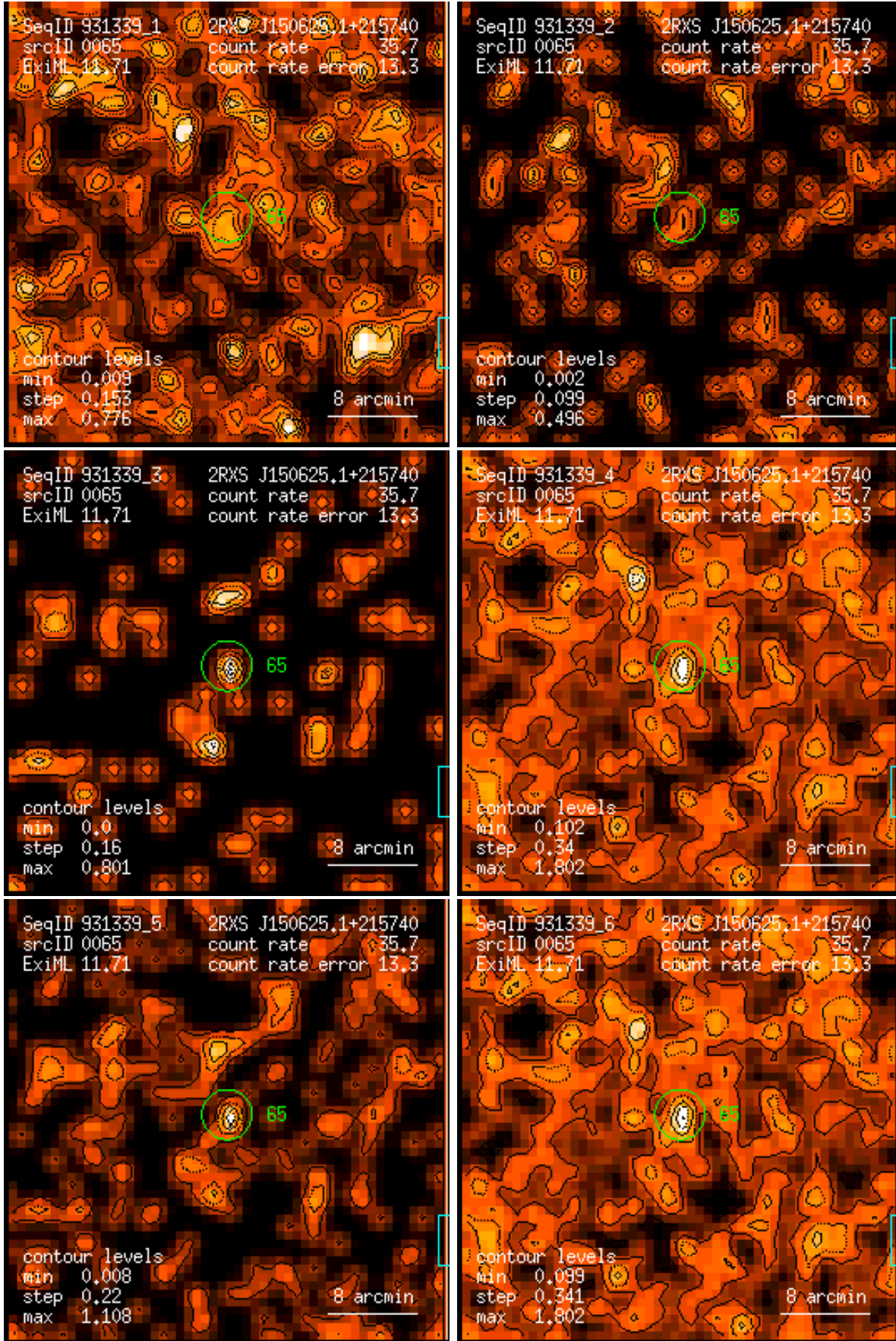
Figure 65: RASS 931339: detection 0065: band rate images, Gaussian filter: (1) PSPC channels 11 – 41, (2) 52 – 90, (3) 91 – 201, (4) 11 – 235, (5) 52 – 201, (6) 11 – 201. Broad band rates in counts/ks. Band rate contour levels in counts/ks/arcmin 2 .
