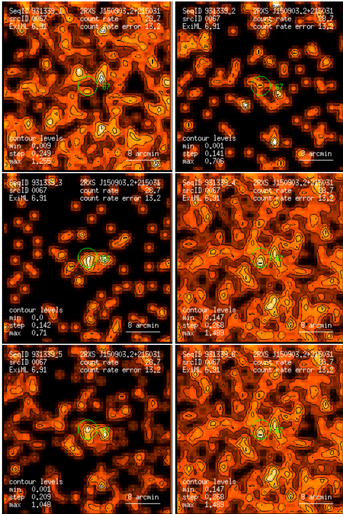
Figure 67: RASS 931339: detection 0067: band rate images, Gaussian filter: (1) PSPC channels 11 – 41, (2) 52 – 90, (3) 91 – 201, (4) 11 – 235, (5) 52 – 201, (6) 11 – 201. Broad band rates in counts/ks. Band rate contour levels in counts/ks/arcmin 2 .
