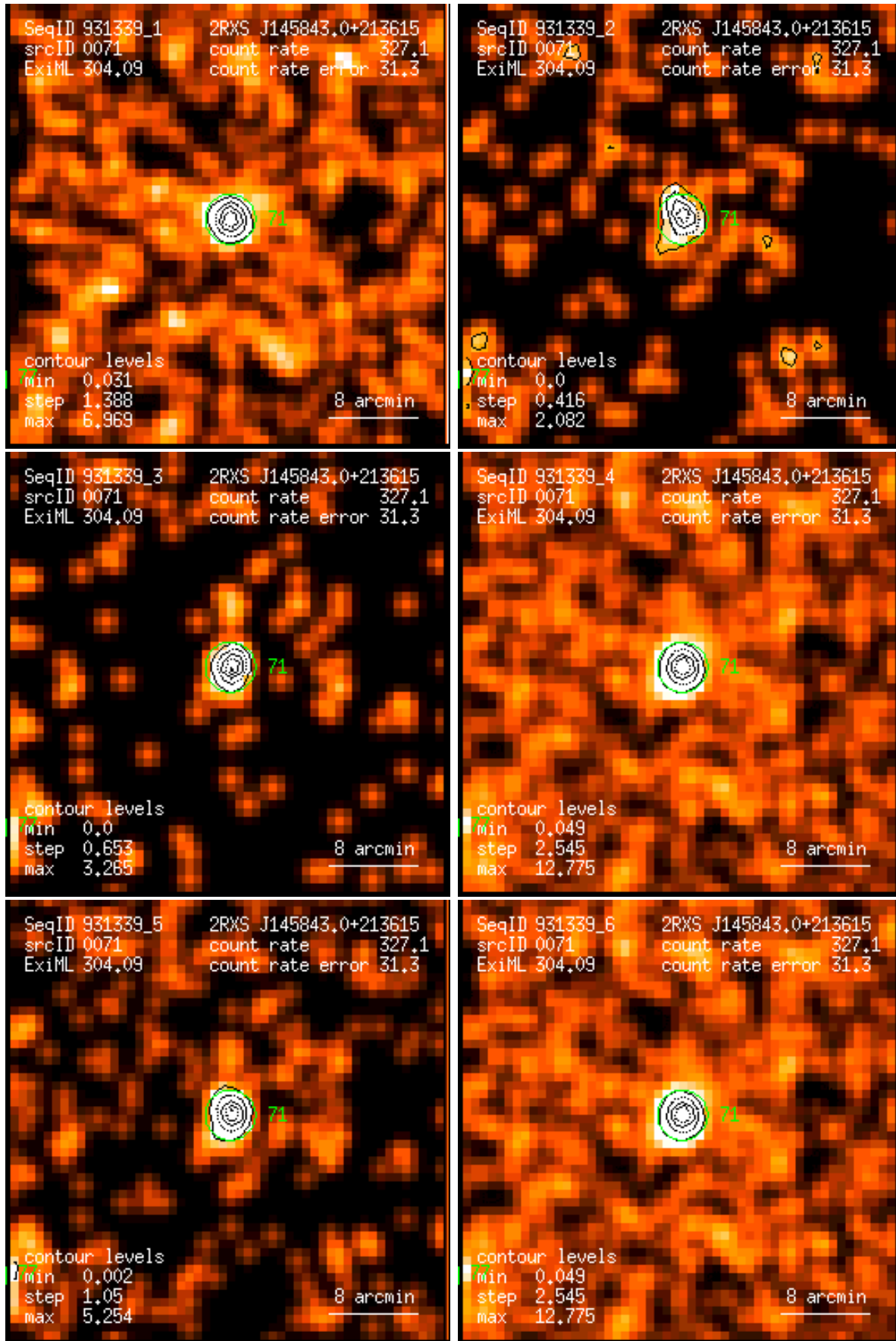
Figure 71: RASS 931339: detection 0071: band rate images, Gaussian filter: (1) PSPC channels 11 – 41, (2) 52 – 90, (3) 91 – 201, (4) 11 – 235, (5) 52 – 201, (6) 11 – 201. Broad band rates in counts/ks. Band rate contour levels in counts/ks/arcmin 2 .
