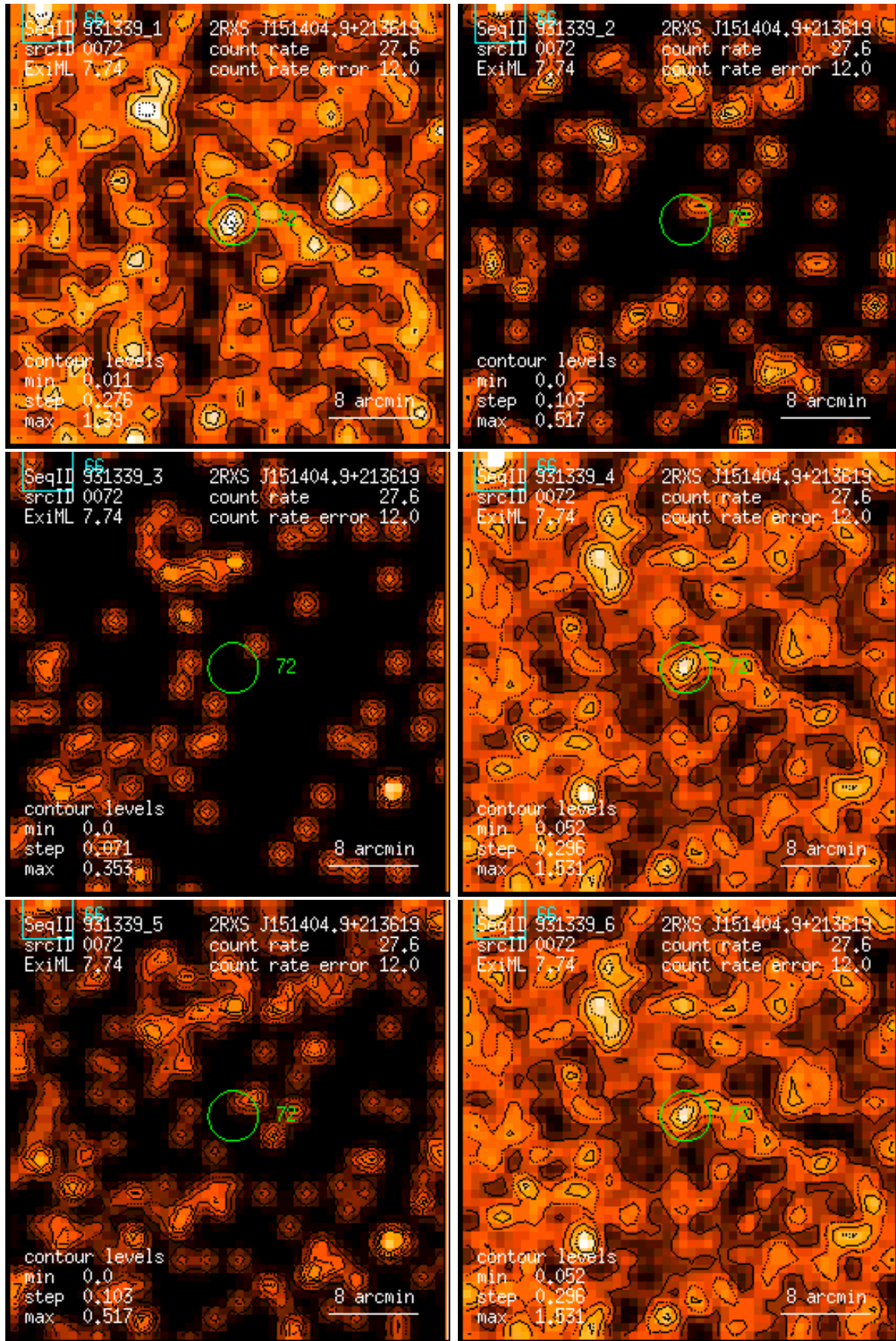
Figure 72: RASS 931339: detection 0072: band rate images, Gaussian filter: (1) PSPC channels 11 – 41, (2) 52 – 90, (3) 91 – 201, (4) 11 – 235, (5) 52 – 201, (6) 11 – 201. Broad band rates in counts/ks. Band rate contour levels in counts/ks/arcmin 2 .
