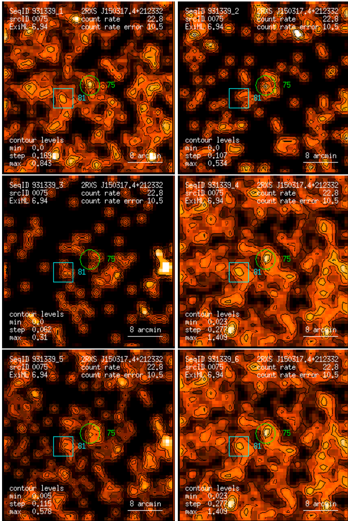
Figure 75: RASS 931339: detection 0075: band rate images, Gaussian filter: (1) PSPC channels 11 – 41, (2) 52 – 90, (3) 91 – 201, (4) 11 – 235, (5) 52 – 201, (6) 11 – 201. Broad band rates in counts/ks. Band rate contour levels in counts/ks/arcmin 2 .
