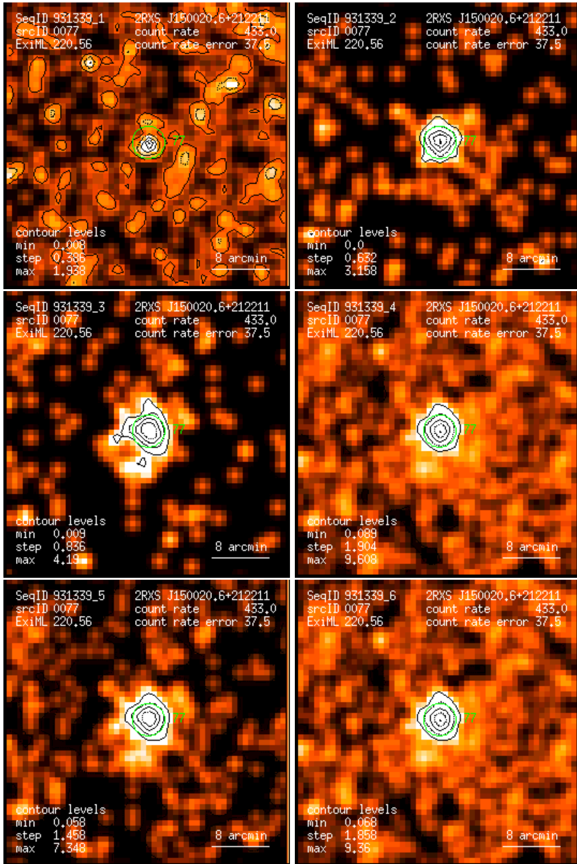
Figure 77: RASS 931339: detection 0077: band rate images, Gaussian filter: (1) PSPC channels 11 – 41, (2) 52 – 90, (3) 91 – 201, (4) 11 – 235, (5) 52 – 201, (6) 11 – 201. Broad band rates in counts/ks. Band rate contour levels in counts/ks/arcmin 2 .
