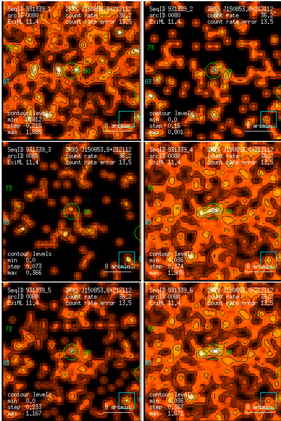
Figure 80: RASS 931339: detection 0080: band rate images, Gaussian filter: (1) PSPC channels 11 – 41, (2) 52 – 90, (3) 91 – 201, (4) 11 – 235, (5) 52 – 201, (6) 11 – 201. Broad band rates in counts/ks. Band rate contour levels in counts/ks/arcmin 2 .
