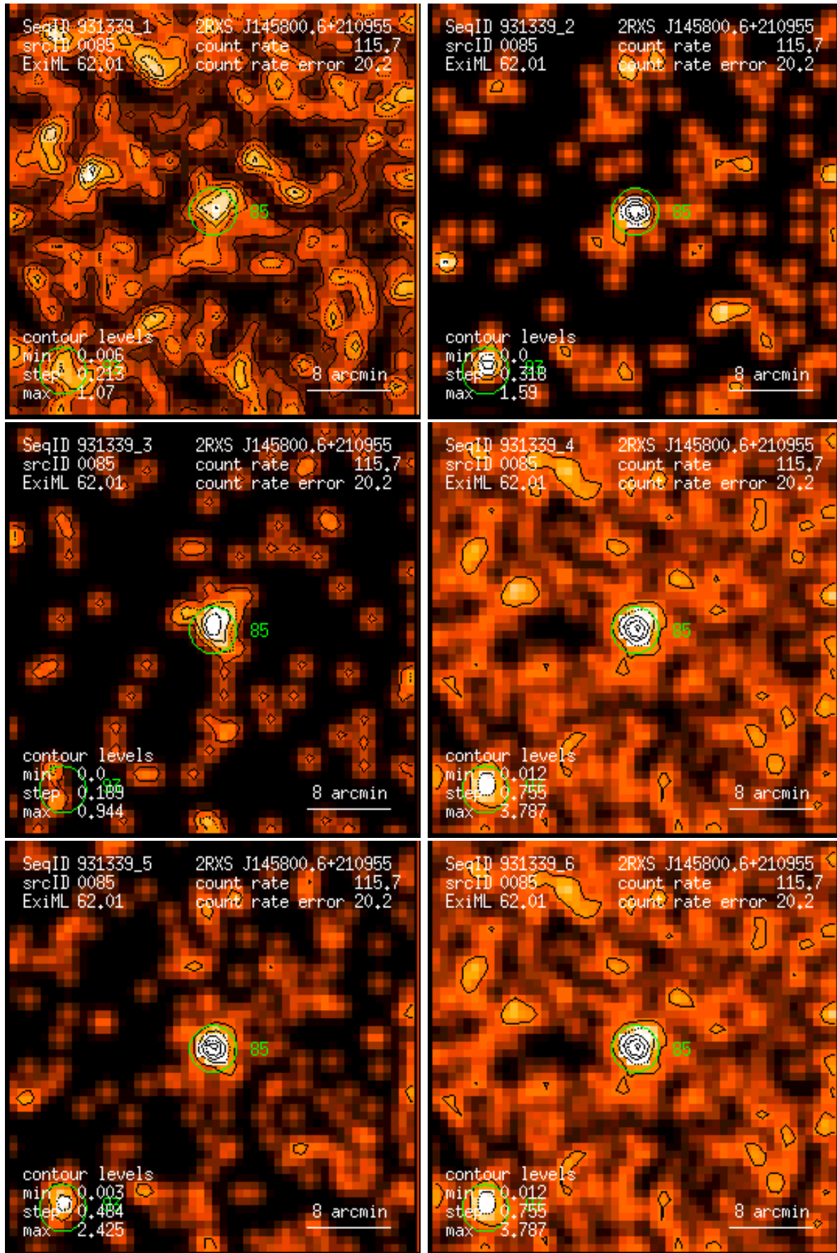
Figure 85: RASS 931339: detection 0085: band rate images, Gaussian filter: (1) PSPC channels 11 – 41, (2) 52 – 90, (3) 91 – 201, (4) 11 – 235, (5) 52 – 201, (6) 11 – 201. Broad band rates in counts/ks. Band rate contour levels in counts/ks/arcmin 2 .
