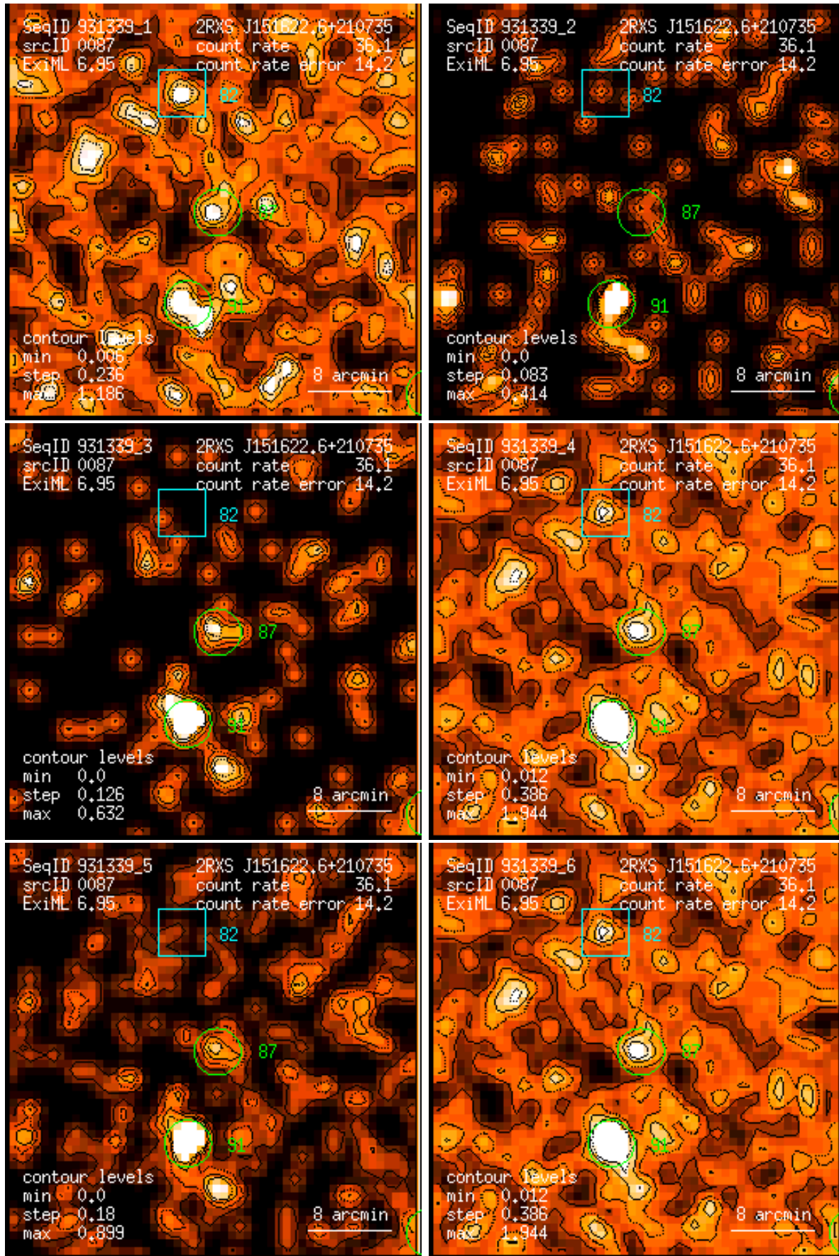
Figure 87: RASS 931339: detection 0087: band rate images, Gaussian filter: (1) PSPC channels 11 – 41, (2) 52 – 90, (3) 91 – 201, (4) 11 – 235, (5) 52 – 201, (6) 11 – 201. Broad band rates in counts/ks. Band rate contour levels in counts/ks/arcmin 2 .
