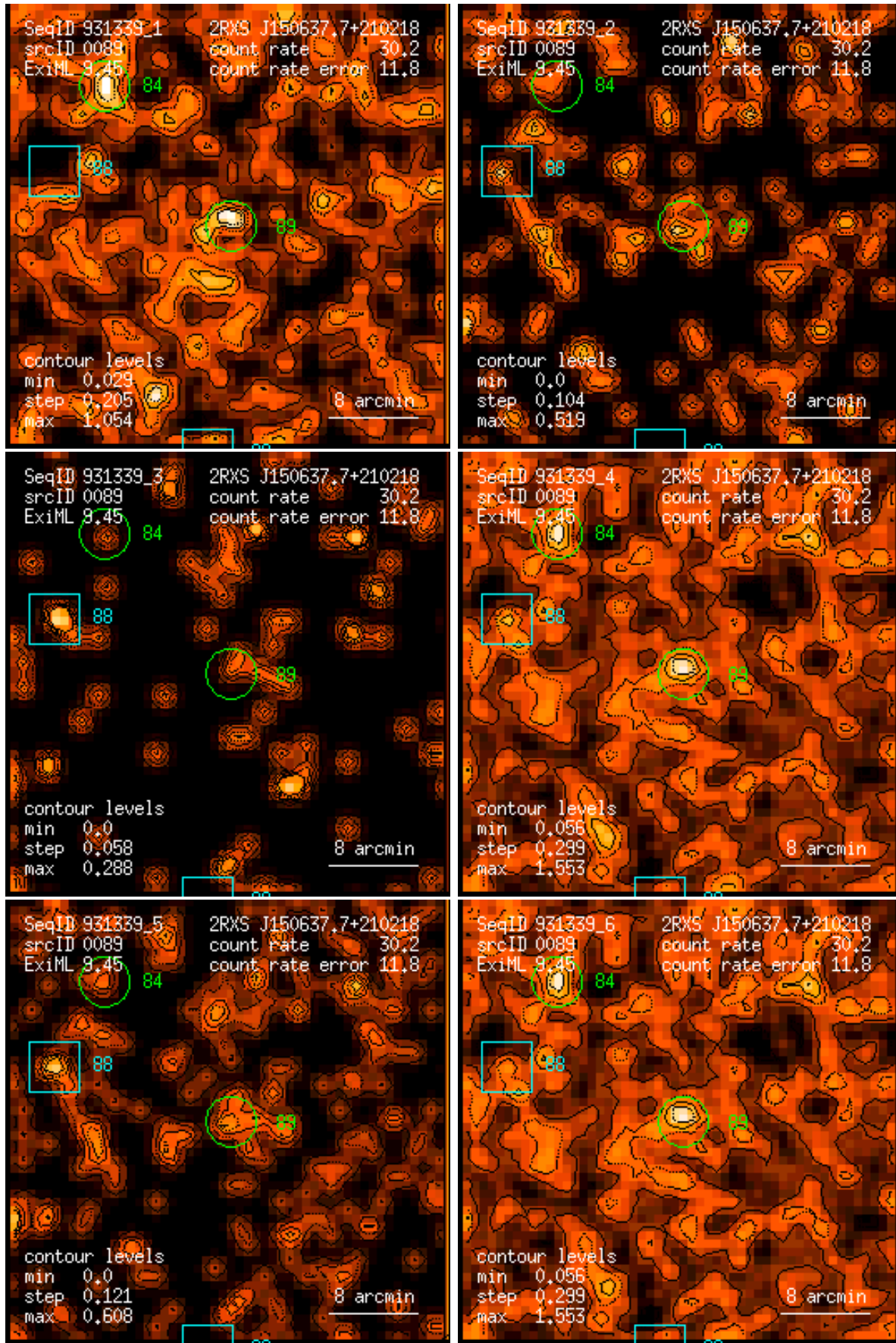
Figure 89: RASS 931339: detection 0089: band rate images, Gaussian filter: (1) PSPC channels 11 – 41, (2) 52 – 90, (3) 91 – 201, (4) 11 – 235, (5) 52 – 201, (6) 11 – 201. Broad band rates in counts/ks. Band rate contour levels in counts/ks/arcmin 2 .
