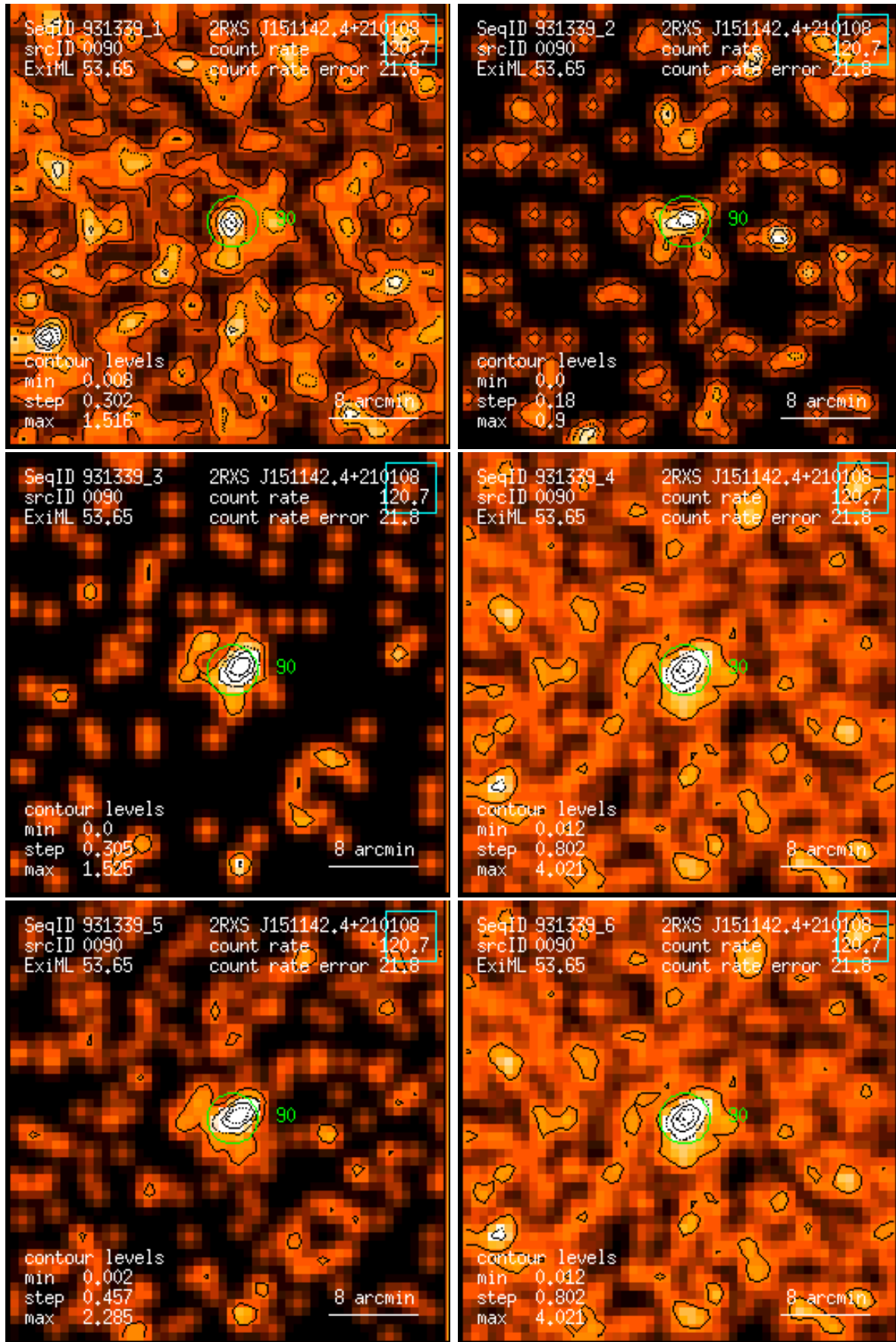
Figure 90: RASS 931339: detection 0090: band rate images, Gaussian filter: (1) PSPC channels 11 – 41, (2) 52 – 90, (3) 91 – 201, (4) 11 – 235, (5) 52 – 201, (6) 11 – 201. Broad band rates in counts/ks. Band rate contour levels in counts/ks/arcmin 2 .
