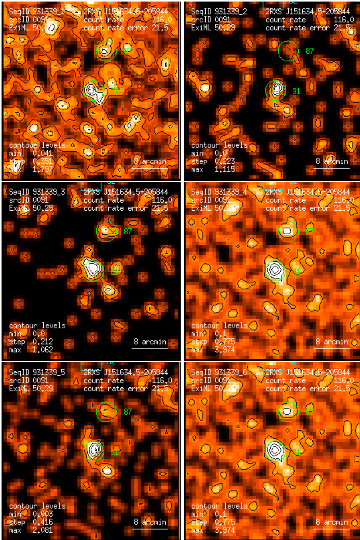
Figure 91: RASS 931339: detection 0091: band rate images, Gaussian filter: (1) PSPC channels 11 – 41, (2) 52 – 90, (3) 91 – 201, (4) 11 – 235, (5) 52 – 201, (6) 11 – 201. Broad band rates in counts/ks. Band rate contour levels in counts/ks/arcmin 2 .
