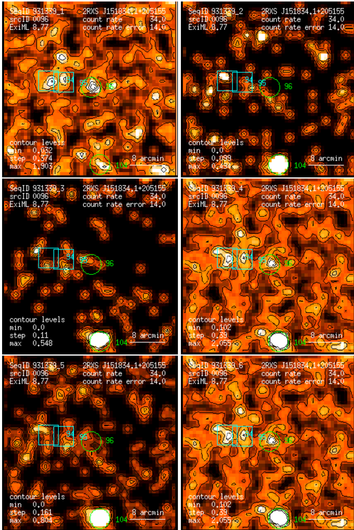
Figure 96: RASS 931339: detection 0096: band rate images, Gaussian filter: (1) PSPC channels 11 – 41, (2) 52 – 90, (3) 91 – 201, (4) 11 – 235, (5) 52 – 201, (6) 11 – 201. Broad band rates in counts/ks. Band rate contour levels in counts/ks/arcmin 2 .
