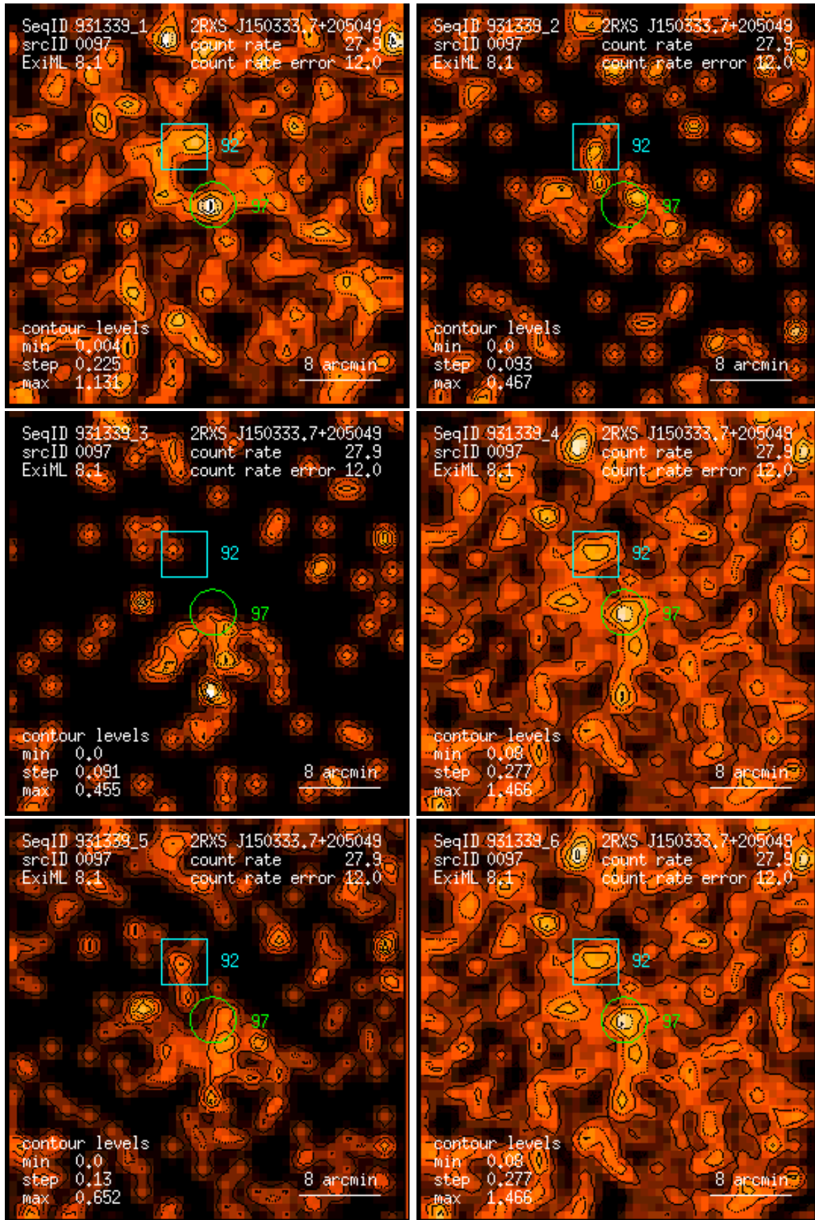
Figure 97: RASS 931339: detection 0097: band rate images, Gaussian filter: (1) PSPC channels 11 – 41, (2) 52 – 90, (3) 91 – 201, (4) 11 – 235, (5) 52 – 201, (6) 11 – 201. Broad band rates in counts/ks. Band rate contour levels in counts/ks/arcmin 2 .
