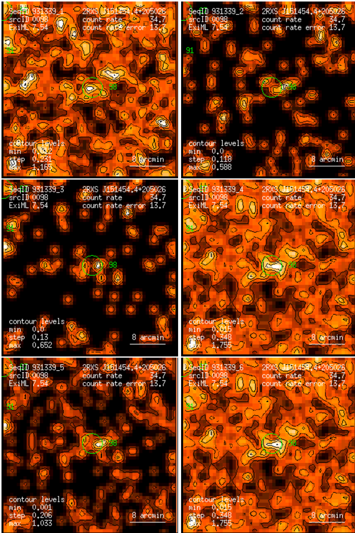
Figure 98: RASS 931339: detection 0098: band rate images, Gaussian filter: (1) PSPC channels 11 – 41, (2) 52 – 90, (3) 91 – 201, (4) 11 – 235, (5) 52 – 201, (6) 11 – 201. Broad band rates in counts/ks. Band rate contour levels in counts/ks/arcmin 2 .
