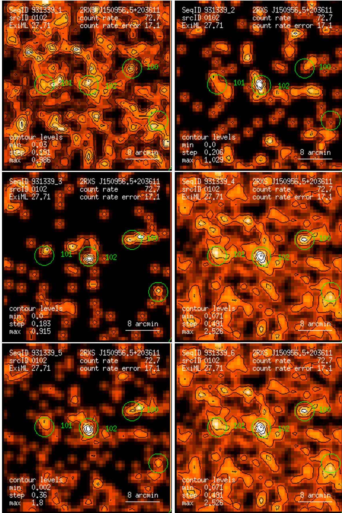
Figure 102: RASS 931339: detection 0102: band rate images, Gaussian filter: (1) PSPC channels 11 – 41, (2) 52 – 90, (3) 91 – 201, (4) 11 – 235, (5) 52 – 201, (6) 11 – 201. Broad band rates in counts/ks. Band rate contour levels in counts/ks/arcmin 2 .
