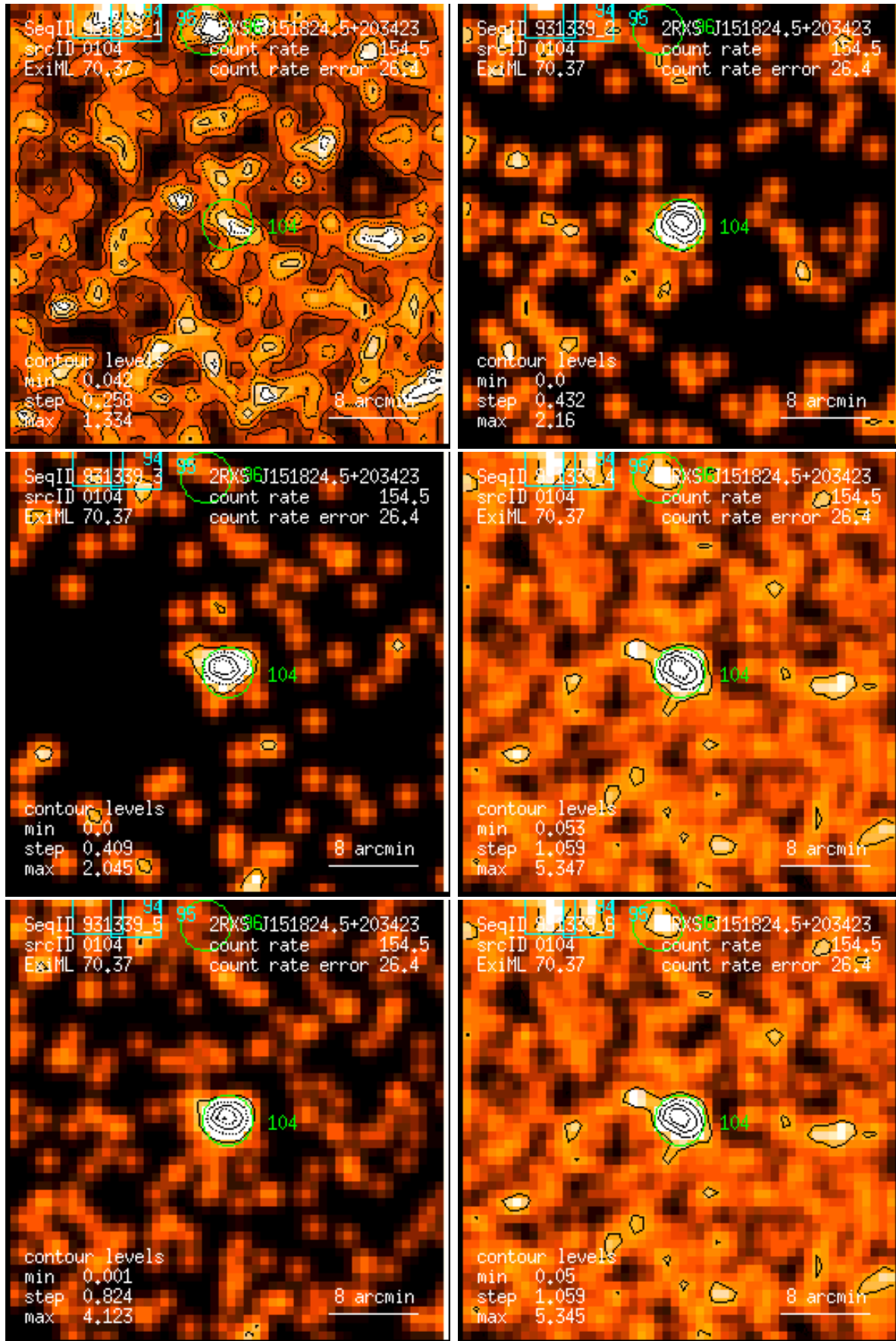
Figure 104: RASS 931339: detection 0104: band rate images, Gaussian filter: (1) PSPC channels 11 – 41, (2) 52 – 90, (3) 91 – 201, (4) 11 – 235, (5) 52 – 201, (6) 11 – 201. Broad band rates in counts/ks. Band rate contour levels in counts/ks/arcmin 2 .
