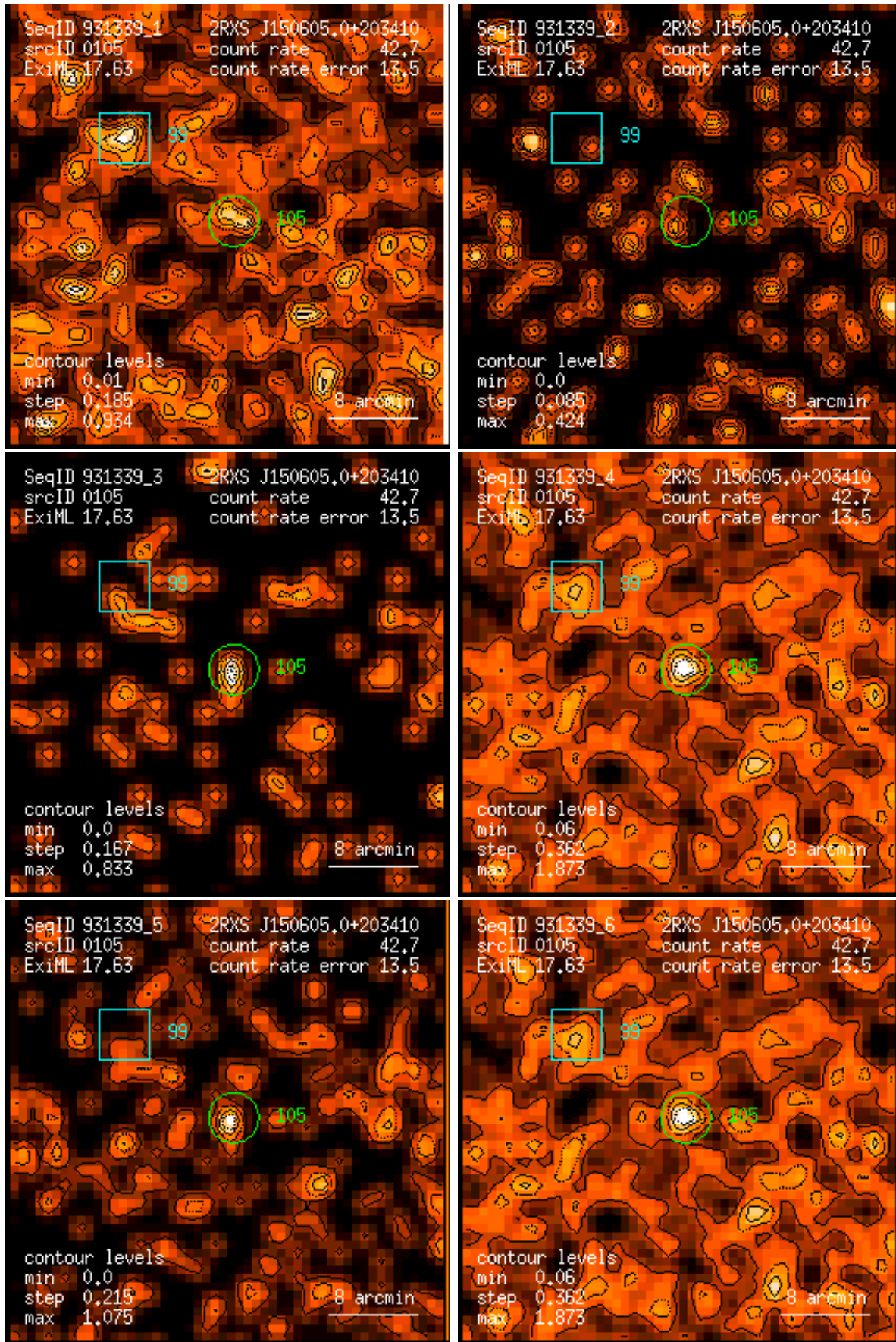
Figure 105: RASS 931339: detection 0105: band rate images, Gaussian filter: (1) PSPC channels 11 – 41, (2) 52 – 90, (3) 91 – 201, (4) 11 – 235, (5) 52 – 201, (6) 11 – 201. Broad band rates in counts/ks. Band rate contour levels in counts/ks/arcmin 2 .
