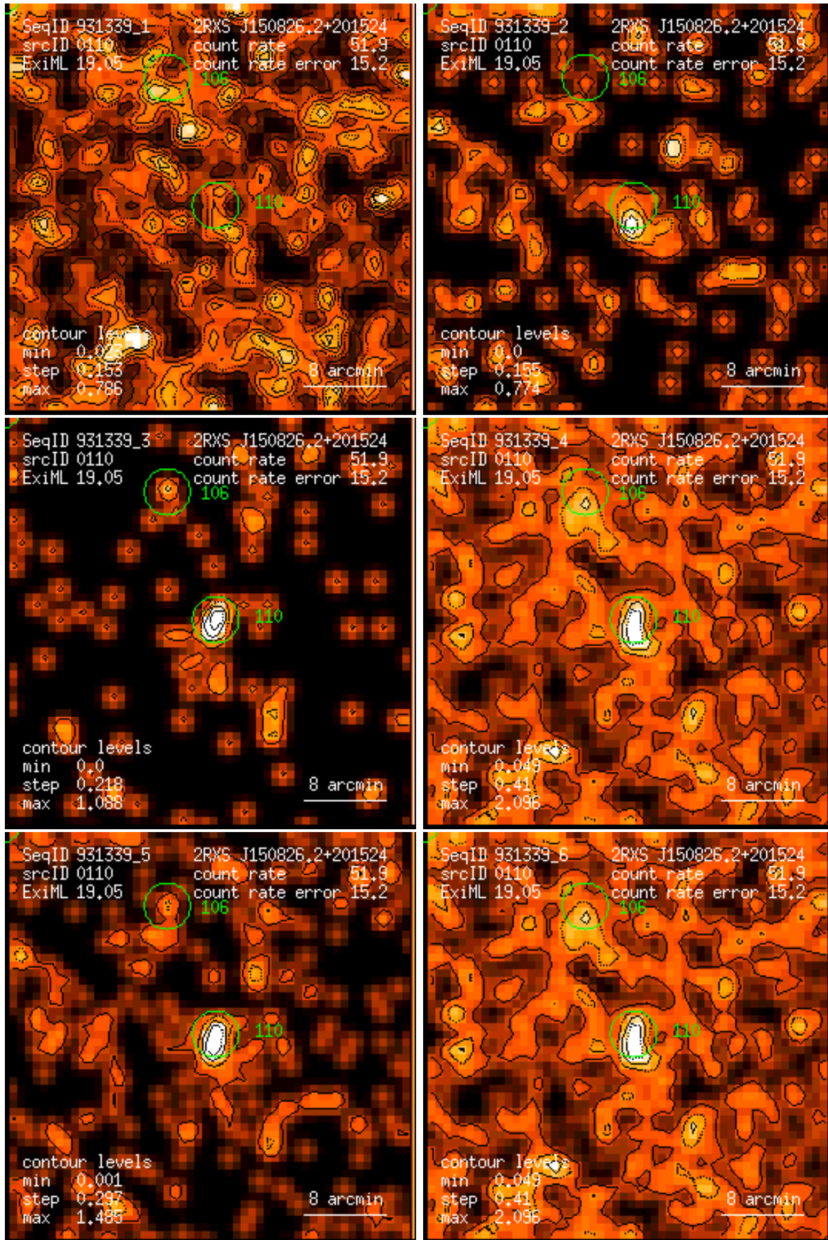
Figure 110: RASS 931339: detection 0110: band rate images, Gaussian filter: (1) PSPC channels 11 – 41, (2) 52 – 90, (3) 91 – 201, (4) 11 – 235, (5) 52 – 201, (6) 11 – 201. Broad band rates in counts/ks. Band rate contour levels in counts/ks/arcmin 2 .
