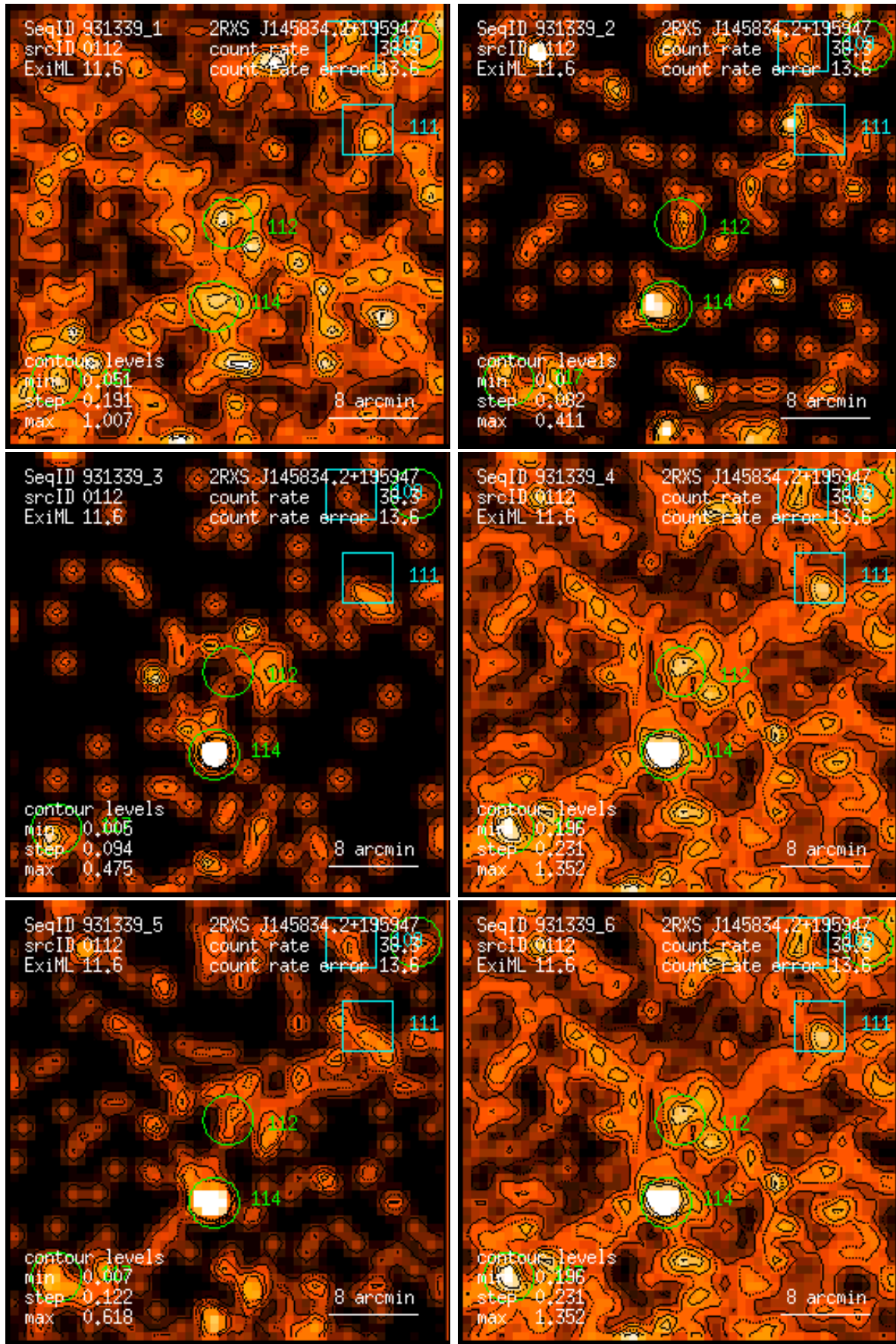
Figure 112: RASS 931339: detection 0112: band rate images, Gaussian filter: (1) PSPC channels 11 – 41, (2) 52 – 90, (3) 91 – 201, (4) 11 – 235, (5) 52 – 201, (6) 11 – 201. Broad band rates in counts/ks. Band rate contour levels in counts/ks/arcmin 2 .
