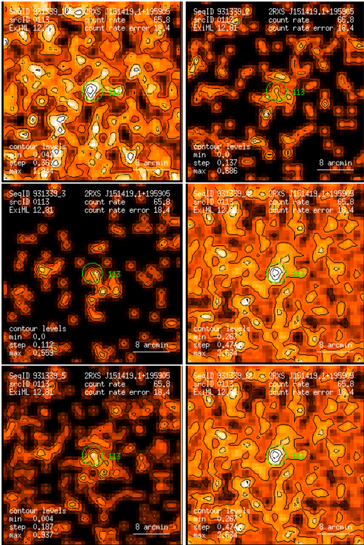
Figure 113: RASS 931339: detection 0113: band rate images, Gaussian filter: (1) PSPC channels 11 – 41, (2) 52 – 90, (3) 91 – 201, (4) 11 – 235, (5) 52 – 201, (6) 11 – 201. Broad band rates in counts/ks. Band rate contour levels in counts/ks/arcmin 2 .
