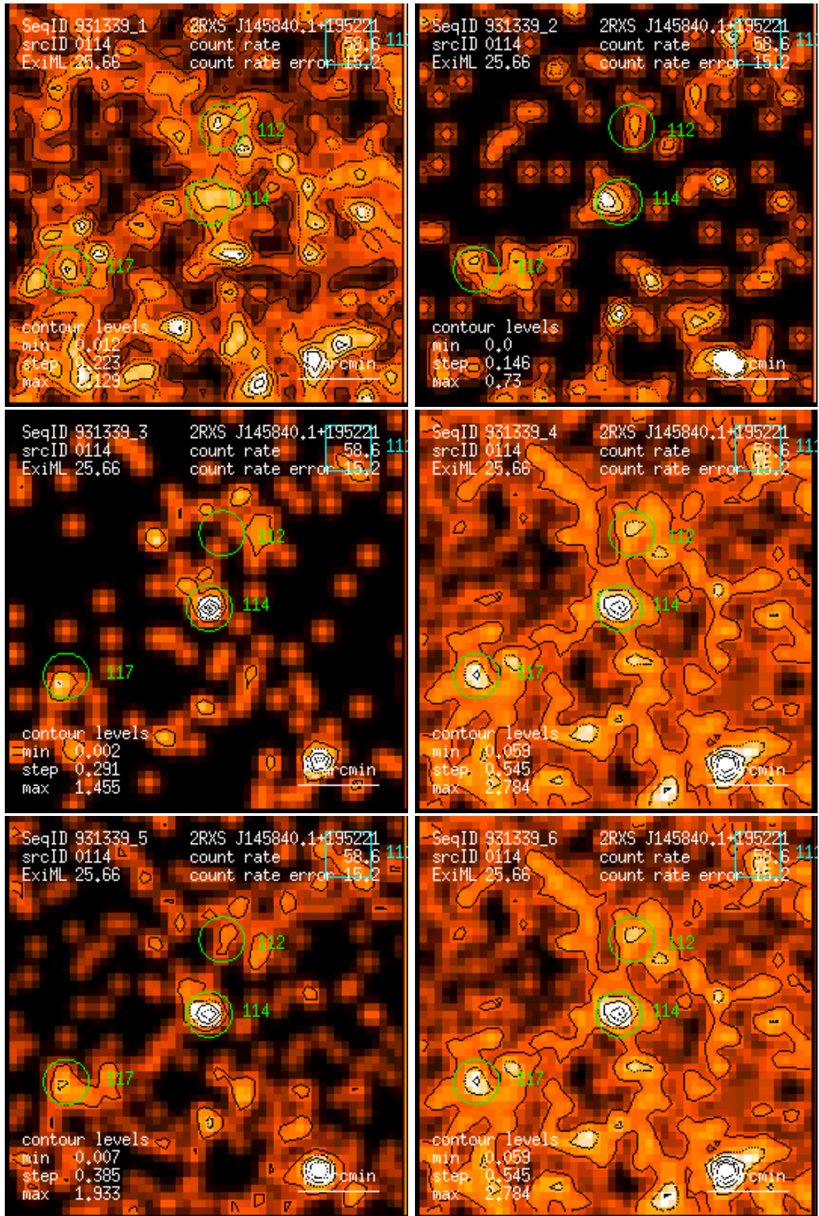
Figure 114: RASS 931339: detection 0114: band rate images, Gaussian filter: (1) PSPC channels 11 – 41, (2) 52 – 90, (3) 91 – 201, (4) 11 – 235, (5) 52 – 201, (6) 11 – 201. Broad band rates in counts/ks. Band rate contour levels in counts/ks/arcmin 2 .
