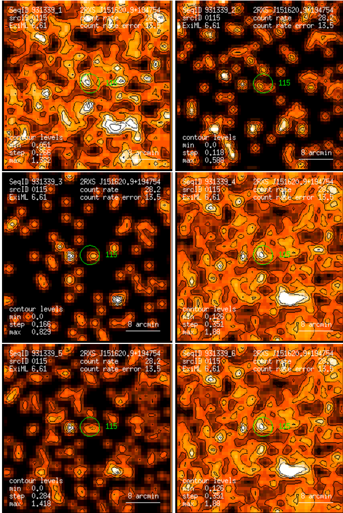
Figure 115: RASS 931339: detection 0115: band rate images, Gaussian filter: (1) PSPC channels 11 – 41, (2) 52 – 90, (3) 91 – 201, (4) 11 – 235, (5) 52 – 201, (6) 11 – 201. Broad band rates in counts/ks. Band rate contour levels in counts/ks/arcmin 2 .
