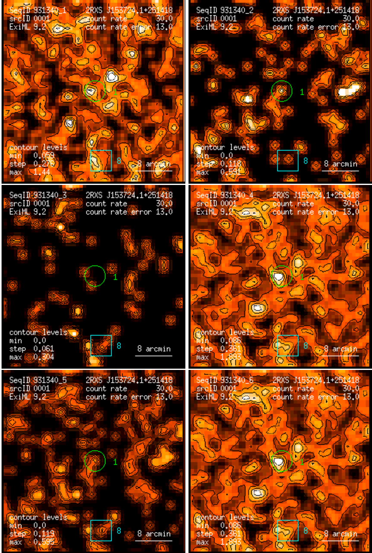
Figure 1: RASS 931340: detection 0001: band rate images, Gaussian filter: (1) PSPC channels 11 – 41, (2) 52 – 90, (3) 91 – 201, (4) 11 – 235, (5) 52 – 201, (6) 11 – 201. Broad band rates in counts/ks. Band rate contour levels in counts/ks/arcmin 2 .
