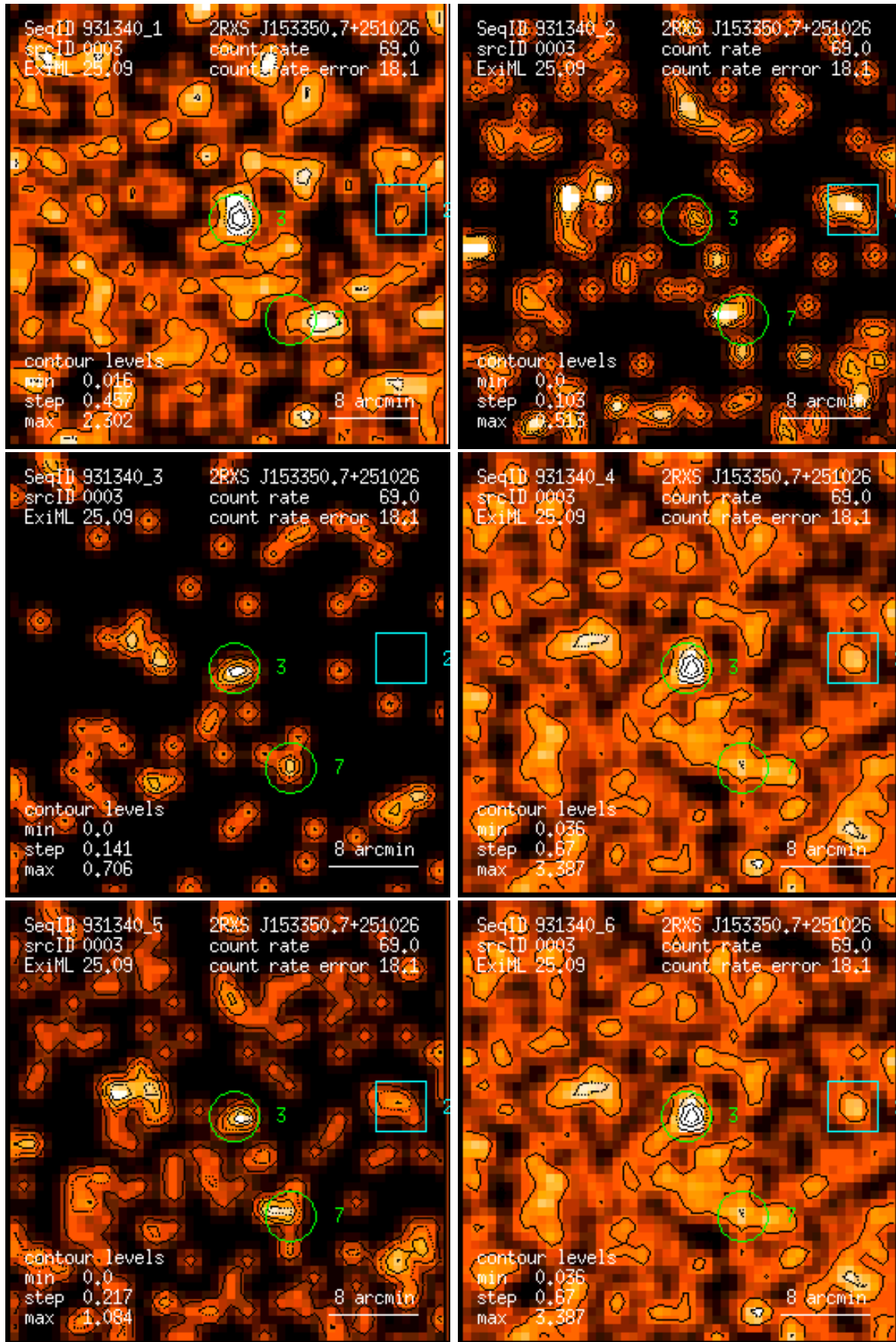
Figure 3: RASS 931340: detection 0003: band rate images, Gaussian filter: (1) PSPC channels 11 – 41, (2) 52 – 90, (3) 91 – 201, (4) 11 – 235, (5) 52 – 201, (6) 11 – 201. Broad band rates in counts/ks. Band rate contour levels in counts/ks/arcmin 2 .
