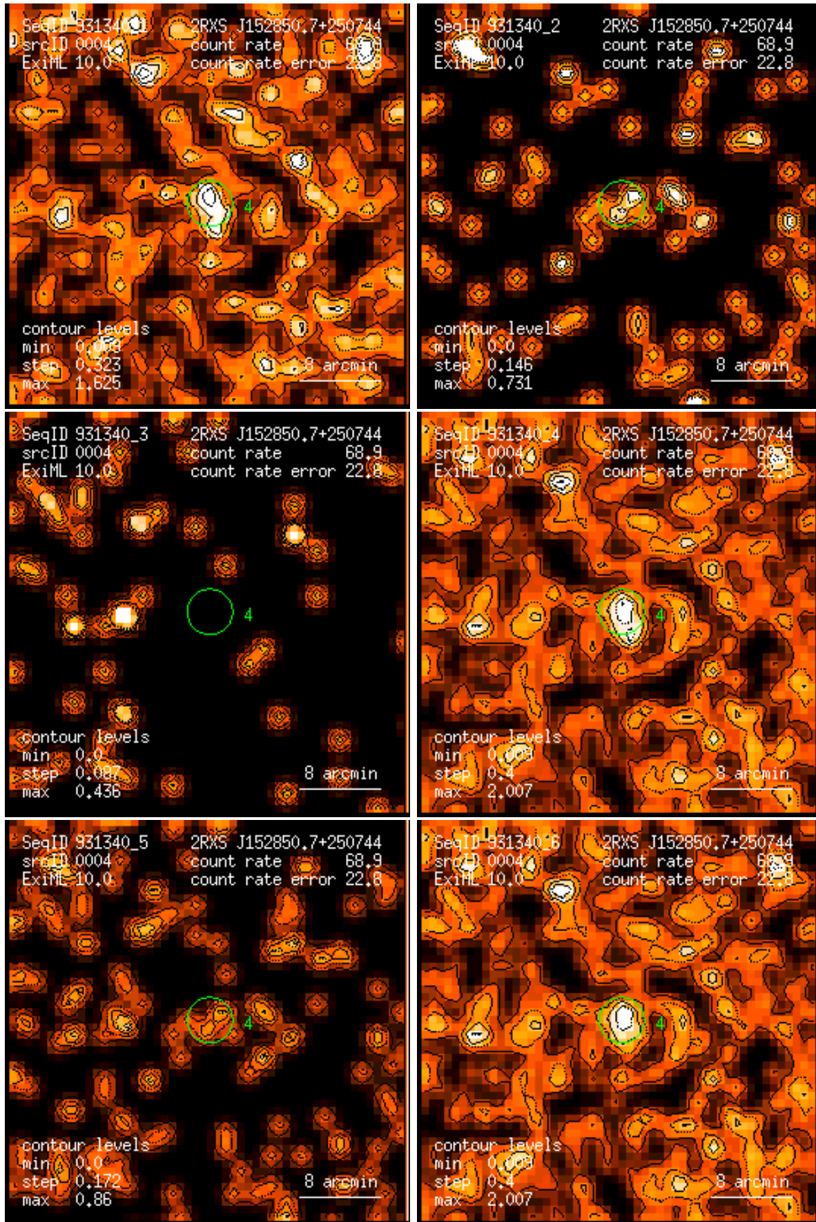
Figure 4: RASS 931340: detection 0004: band rate images, Gaussian filter: (1) PSPC channels 11 – 41, (2) 52 – 90, (3) 91 – 201, (4) 11 – 235, (5) 52 – 201, (6) 11 – 201. Broad band rates in counts/ks. Band rate contour levels in counts/ks/arcmin 2 .
