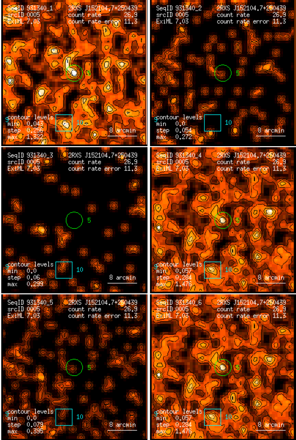
Figure 5: RASS 931340: detection 0005: band rate images, Gaussian filter: (1) PSPC channels 11 – 41, (2) 52 – 90, (3) 91 – 201, (4) 11 – 235, (5) 52 – 201, (6) 11 – 201. Broad band rates in counts/ks. Band rate contour levels in counts/ks/arcmin 2 .
