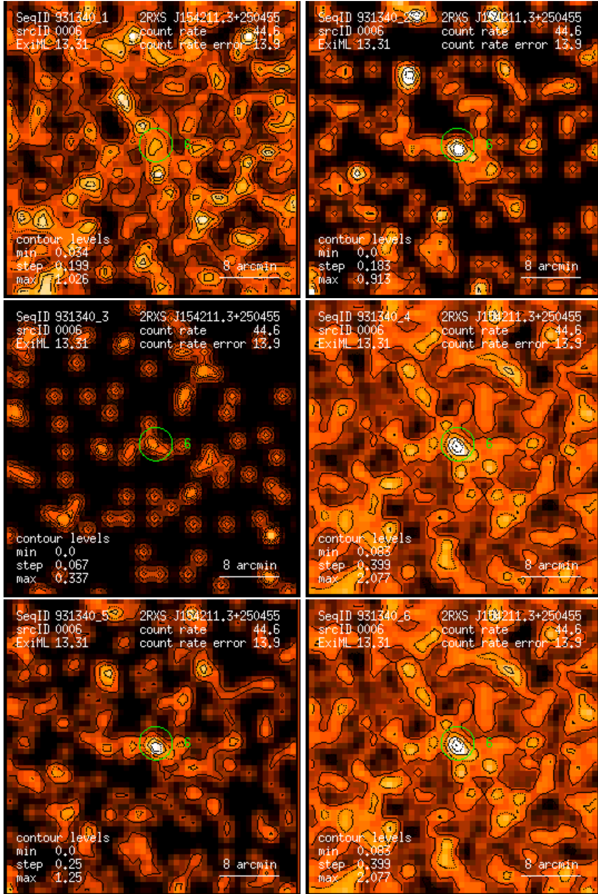
Figure 6: RASS 931340: detection 0006: band rate images, Gaussian filter: (1) PSPC channels 11 – 41, (2) 52 – 90, (3) 91 – 201, (4) 11 – 235, (5) 52 – 201, (6) 11 – 201. Broad band rates in counts/ks. Band rate contour levels in counts/ks/arcmin 2 .
