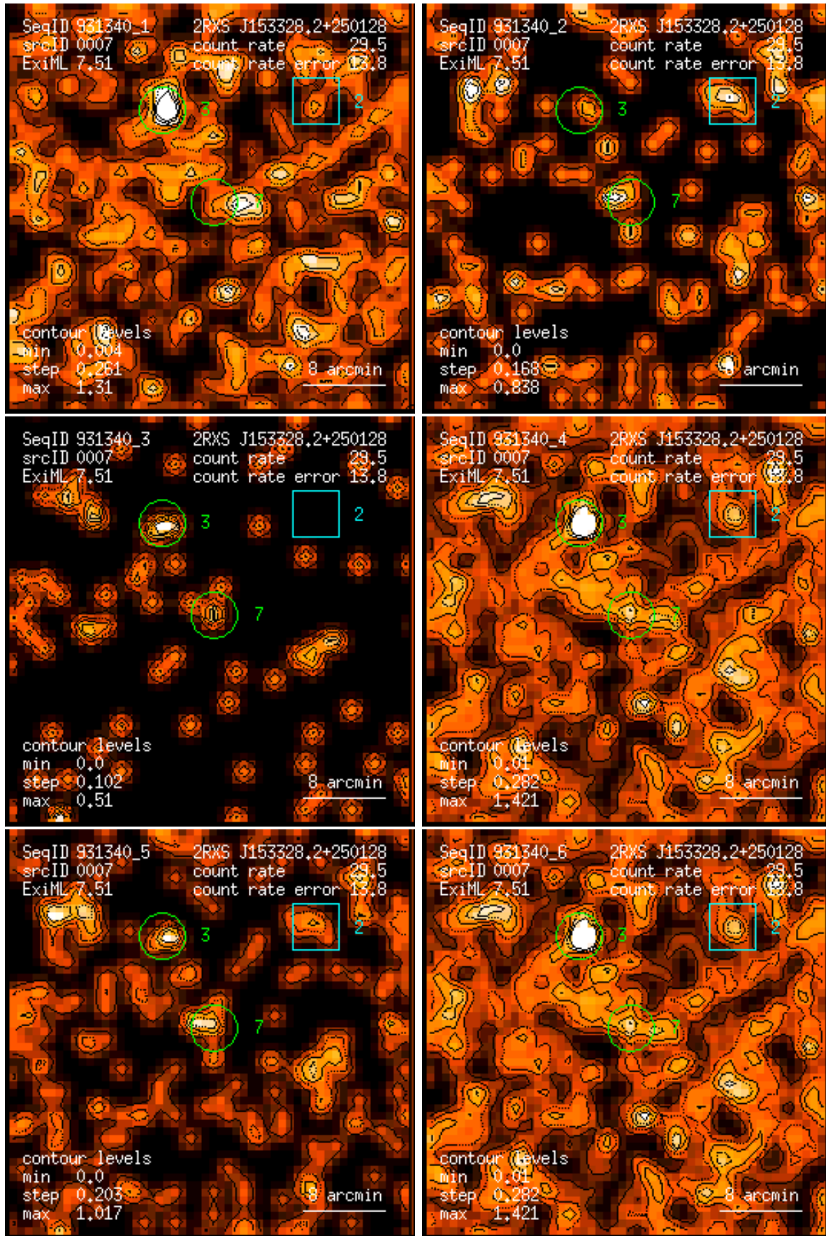
Figure 7: RASS 931340: detection 0007: band rate images, Gaussian filter: (1) PSPC channels 11 – 41, (2) 52 – 90, (3) 91 – 201, (4) 11 – 235, (5) 52 – 201, (6) 11 – 201. Broad band rates in counts/ks. Band rate contour levels in counts/ks/arcmin 2 .
