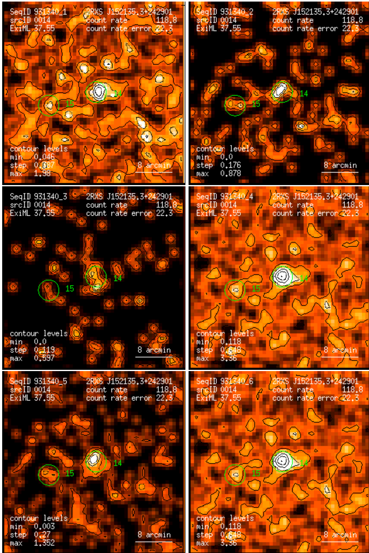
Figure 14: RASS 931340: detection 0014: band rate images, Gaussian filter: (1) PSPC channels 11 – 41, (2) 52 – 90, (3) 91 – 201, (4) 11 – 235, (5) 52 – 201, (6) 11 – 201. Broad band rates in counts/ks. Band rate contour levels in counts/ks/arcmin 2 .
