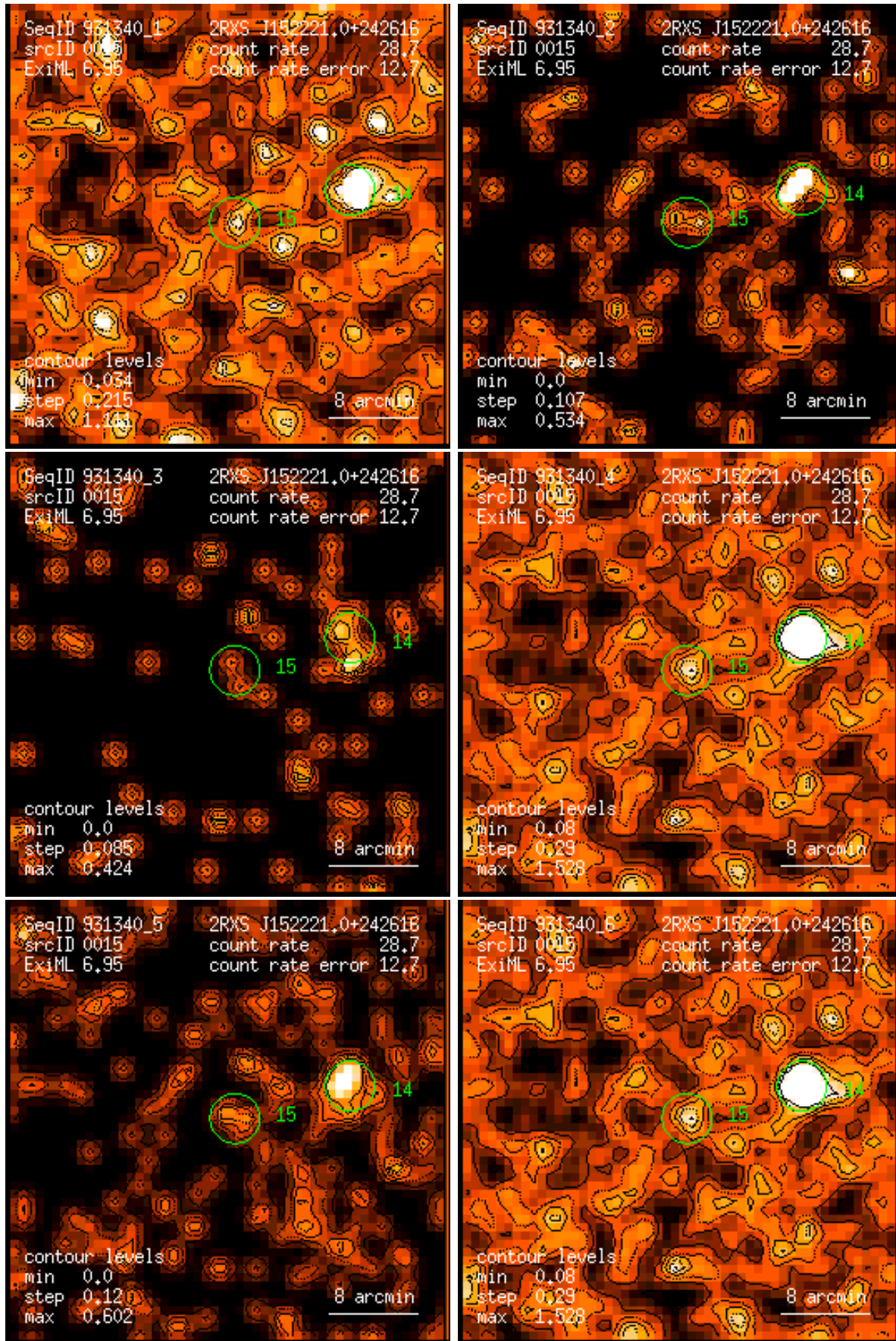
Figure 15: RASS 931340: detection 0015: band rate images, Gaussian filter: (1) PSPC channels 11 – 41, (2) 52 – 90, (3) 91 – 201, (4) 11 – 235, (5) 52 – 201, (6) 11 – 201. Broad band rates in counts/ks. Band rate contour levels in counts/ks/arcmin 2 .
