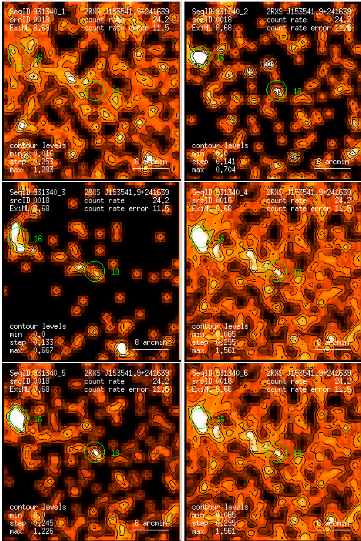
Figure 18: RASS 931340: detection 0018: band rate images, Gaussian filter: (1) PSPC channels 11 – 41, (2) 52 – 90, (3) 91 – 201, (4) 11 – 235, (5) 52 – 201, (6) 11 – 201. Broad band rates in counts/ks. Band rate contour levels in counts/ks/arcmin 2 .
